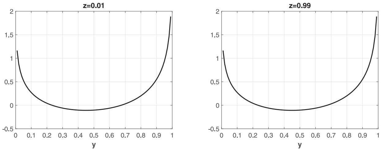
Fig. 2. Plot of Eq. (7.4) written in the form g(y) = 0 , for p = 10 , q = 15 , x = 4.5 and z = 0.01, 0.99 ( z as in (7.1) and (7.3)).
