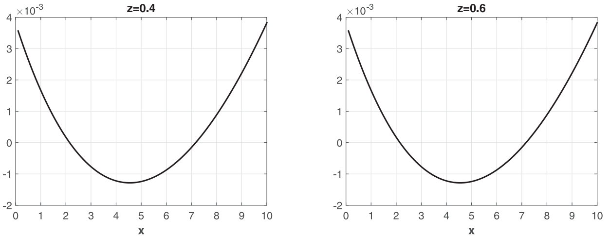
Fig. 1. Plot of Eq. (7.4) written in the form f(x) = 0 , for p = 10 , q = 15 , y = 0.45 and z = 0.4, 0.6 ( z as in (7.1) and (7.3)).
