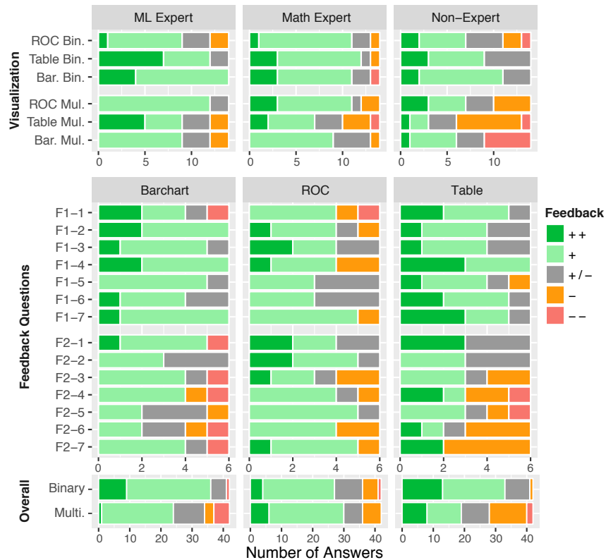
Fig. 16. User feedback.
