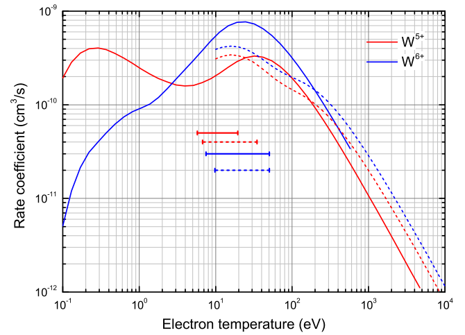
Fig. 1. Total DR rate coefficients for W^{5+} [32] of the [Kr]4d^{10}4f^{14}5s^25p^65d ground level and W^{6+} [33] of the [Kr]4d^{10}4f^{14}5s^25p^6 ground level. The colored short dashed lines represent the corresponding ADAS DR rate coefficients. The horizontal bars indicate the temperature region of formation for each ion where fractional abundance is over 1%. The solid horizontal bars represent the fractional abundance calculation using the present recommended DR data set and the dotted horizontal bars the fractional abundance calculation using the currently available ADAS total recombination data set. See the text of Section 3.13 for more details. (For interpretation of the references to color in this figure legend, the reader is referred to the web version of this article.)
