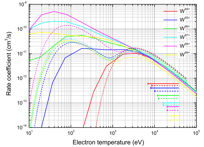
Fig. 9. Total DR rate coefficients for W^{q+} ( q = 64-69 ) of the [\text{He}]2s^22p^m ( m = 6-1 ) ground level [58]. The solid and dotted horizontal bars represent the same as in Fig. 1. (For interpretation of the references to color in this figure legend, the reader is referred to the web version of this article.)
