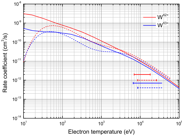
Fig. 8. Total DR rate coefficients for W^{q+} ( q = 62-63 ) of the [\text{Ne}]3s^m ( m = 2-1 ) ground level [58]. The solid and dotted horizontal bars represent the same as in Fig. 1. (For interpretation of the references to color in this figure legend, the reader is referred to the web version of this article.)
