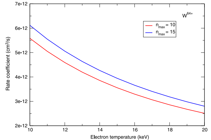
Fig. 12. Total DR rate coefficient for W^{64+} calculated at an electron density of n_e = 10^{14} \text{ cm}^{-3} . The lower red curve represents a model with n_{\text{max}} = 10 and the higher blue curve represents an n_{\text{max}} = 15 model.
