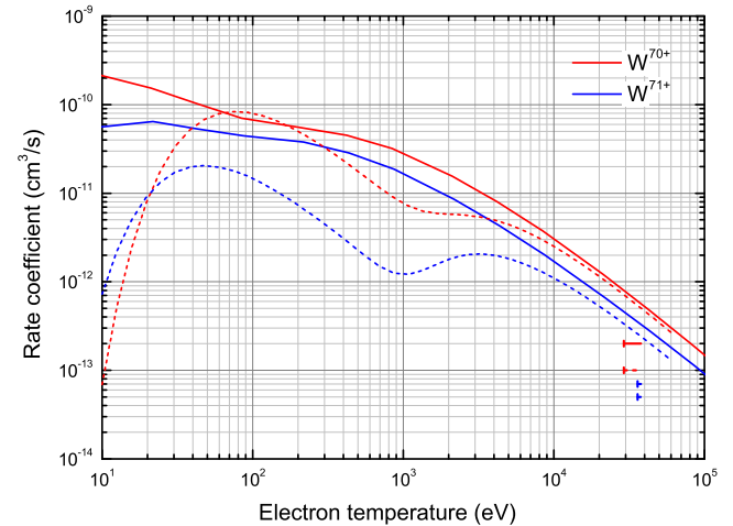
Fig. 10. Total DR rate coefficients for W^{q+} ( q = 70-71 ) of the [\text{He}]2s^m ( m = 2-1 ) ground level [58]. The solid and dotted horizontal bars represent the same as in Fig. 1.
