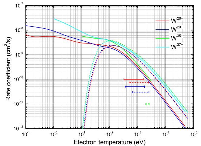
Fig. 3. Total DR rate coefficients for W^{28+} [43] of the [\text{Kr}]4d^{10} ground level, W^{29+} [43] of the [\text{Kr}]4d^9 ground level, W^{35+} [29] of the [\text{Kr}]4d^3 ground level, and W^{37+} [45] of the [\text{Kr}]4d ground level. The solid and dotted horizontal bars represent the same as in Fig. 1. (For interpretation of the references to color in this figure legend, the reader is referred to the web version of this article.)
