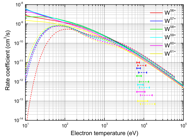
Fig. 7. Total DR rate coefficients for W^{q+} ( q = 56-61 ) of the [Ne]3s^23p^m ( m = 6-1 ) ground level [58]. The solid and dotted horizontal bars represent the same as in Fig. 1. (For interpretation of the references to color in this figure legend, the reader is referred to the web version of this article.)
