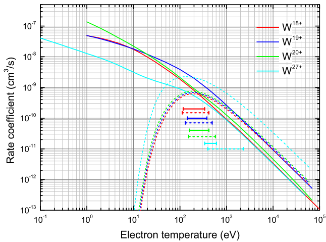
Fig. 2. Total DR rate coefficients for W^{18+} [36,40] of the [\text{Kr}]4d^{10}4f^{10} ground level, W^{19+} [37] of the [\text{Kr}]4d^{10}4f^9 ground level, W^{20+} [38,41] of the [\text{Kr}]4d^{10}4f^8 ground level, and W^{27+} [42] of the [\text{Kr}]4d^{10}4f ground level. The solid and dotted horizontal bars represent the same as in Fig. 1. (For interpretation of the references to color in this figure legend, the reader is referred to the web version of this article.)
