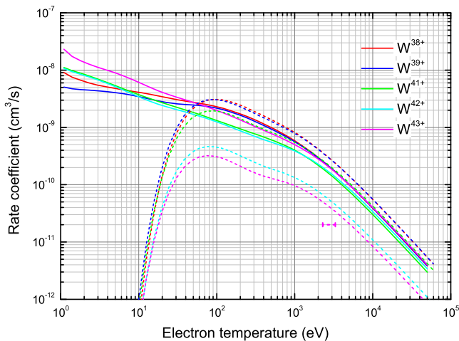
Fig. 4. Total DR rate coefficients for W^{38+} of the [\text{Ar}]3d^{10}4s^24p^6 ground level, W^{39+} of the [\text{Ar}]3d^{10}4s^24p^5 , W^{41+} of the [\text{Ar}]3d^{10}4s^24p^3 ground level, W^{42+} of the [\text{Ar}]3d^{10}4s^24p^2 ground level, and W^{43+} of the [\text{Ar}]3d^{10}4s^24p ground level [47]. The solid and dotted horizontal bars represent the same as in Fig. 1. (For interpretation of the references to color in this figure legend, the reader is referred to the web version of this article.)
