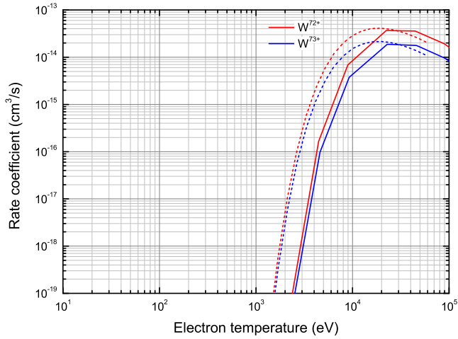
Fig. 11. Total DR rate coefficients for W^{q+} ( q = 72-73 ) of the 1s^m ( m = 2 - 1 ) ground level [58].
