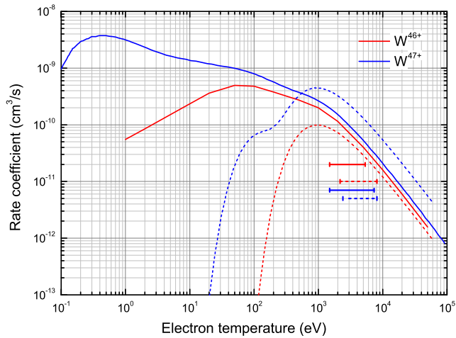
Fig. 6. Total DR rate coefficients for W^{46+} [55] of the [Ar]3d^{10} ground level and for W^{47+} [46] of the [Ar]3d^9 ground level. The dotted horizontal bars represent the same as in Fig. 1. (For interpretation of the references to color in this figure legend, the reader is referred to the web version of this article.)
