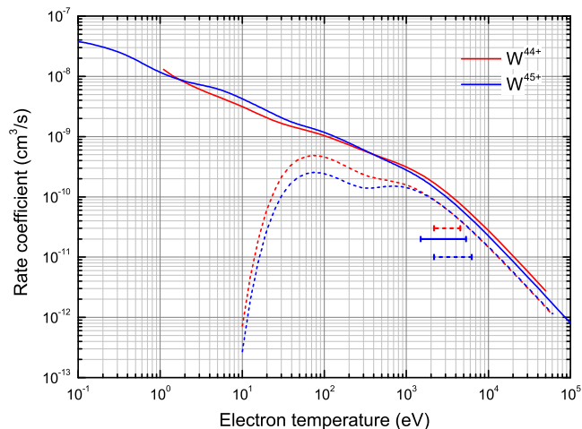
Fig. 5. Total DR rate coefficients for W^{44+} [47] of the [\text{Ar}]3d^{10}4s^2 ground level and for W^{45+} [50–52] of the [\text{Ar}]3d^{10}4s ground level. The colored short dashed lines and the horizontal bars represent same as in Fig. 1. (For interpretation of the references to color in this figure legend, the reader is referred to the web version of this article.)
