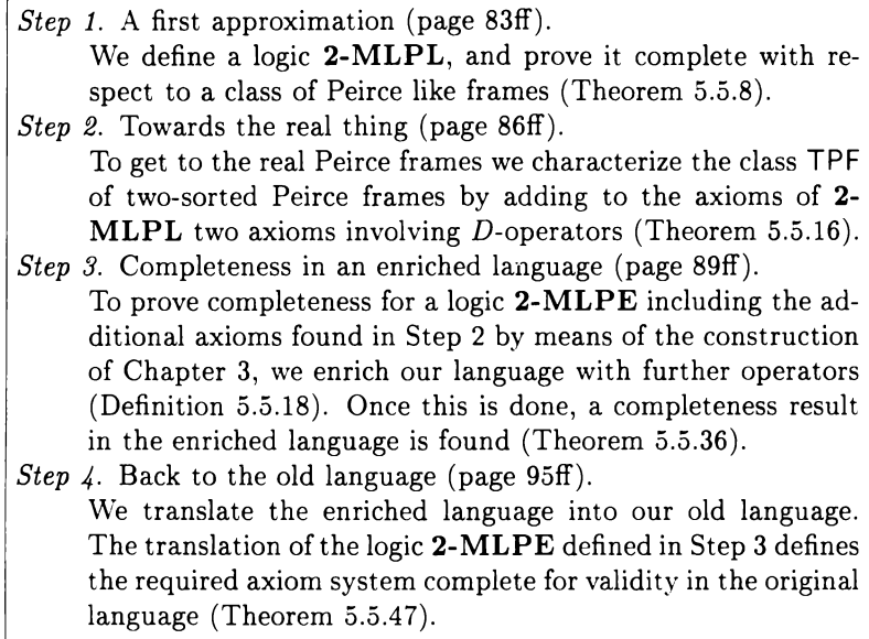
Figure 5.1: A guide to the completeness proof.
