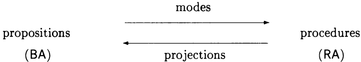
Figure 4.1: Propositions and procedures.
