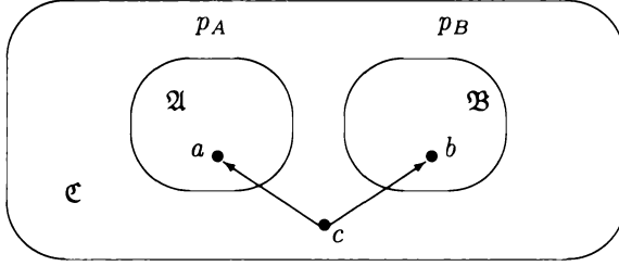
Figure 6.2: Combining models.
