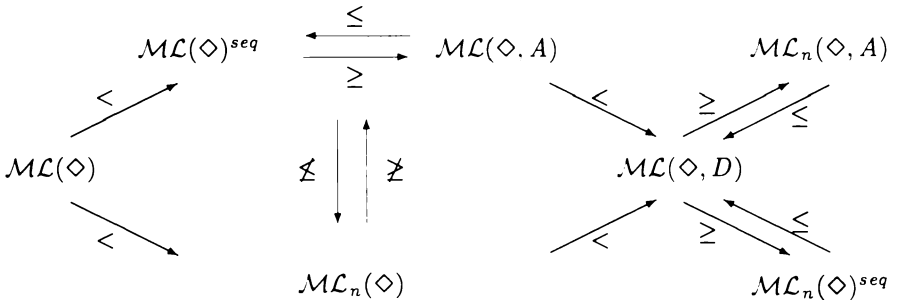
Figure 3.1: \mathcal{ML}(\diamond, D) and its neighbours.
