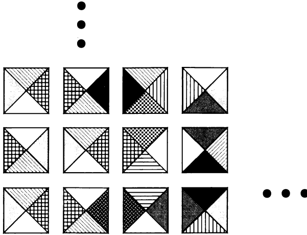
Figure 4.3: An unbounded tiling.
