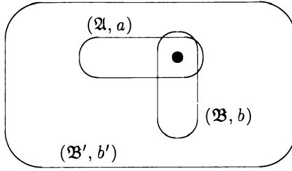
Figure 6.3: Combining (\mathfrak{A}, a) and (\mathfrak{B}, b) .
