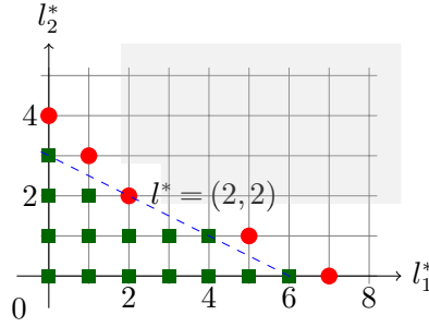
FIGURE 1. An example of important notations introduced in Section 2.1. For (\beta_1 - 1)/(\beta_2 - 1) = 2 and (l_1^*, l_2^*) = (2, 2) , we mark the elements in I_{<(l_1^*, l_2^*)} and J_{(l_1^*, l_2^*)} with squares and circles, respectively. Moreover, the shaded area contains all those points (l_1, l_2) such that (l_1^*, l_2^*) \prec (l_1, l_2) .
