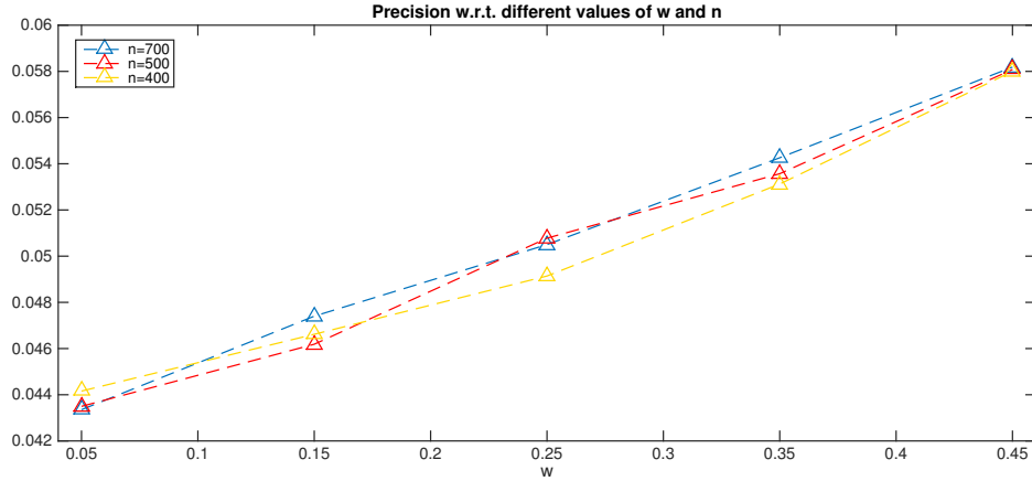
FIGURE 2. A plot of the precision of the estimators discussed in Section 5 w.r.t. w for different values of n .
