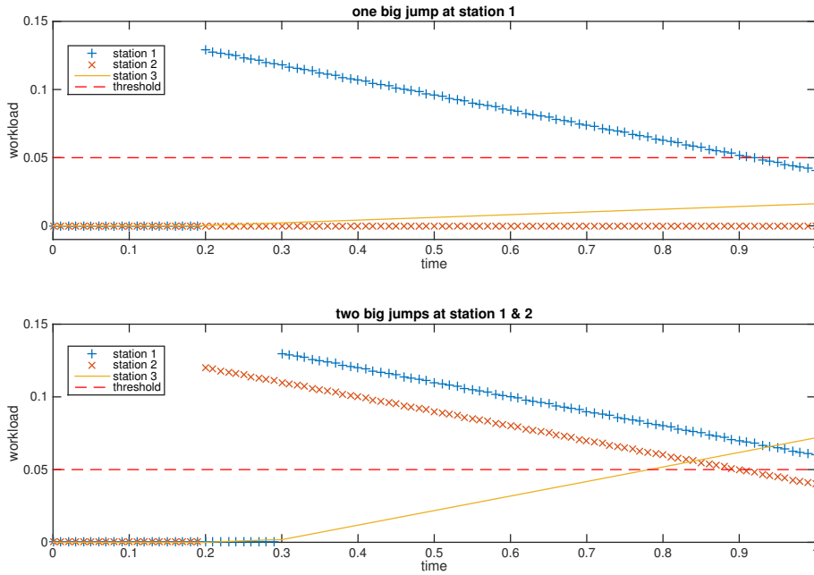
FIGURE 3. An illustration of two different sample paths of workload processes (under the setting of Example 1), whose associated input processes have the form as in (6.5).
