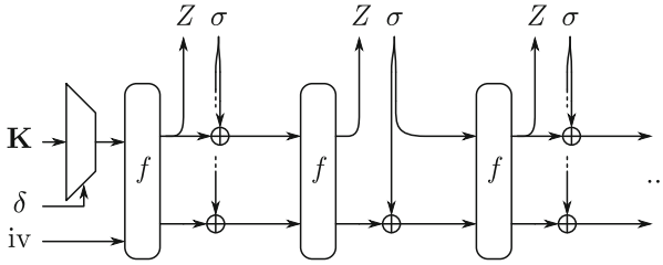
Fig. 1. Full-state keyed duplex construction KD_{\mathbf{K}}^f . In this figure, the sequence of calls is Z = \text{KD.Init}(\delta, \text{iv}, \sigma, \text{false}) , Z = \text{KD.Duplexing}(\sigma, \text{true}) , and Z = \text{KD.Duplexing}(\sigma, \text{false}) .
