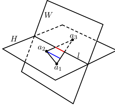
Figure 3: \mathbf{a}_1, \dots, \mathbf{a}_d are conditioned for \text{conv}(\mathbf{a}_1, \dots, \mathbf{a}_d) to intersect W and lie in H . The red line corresponds to induced edge. The blue line represents the longest chord parallel to \ell .
