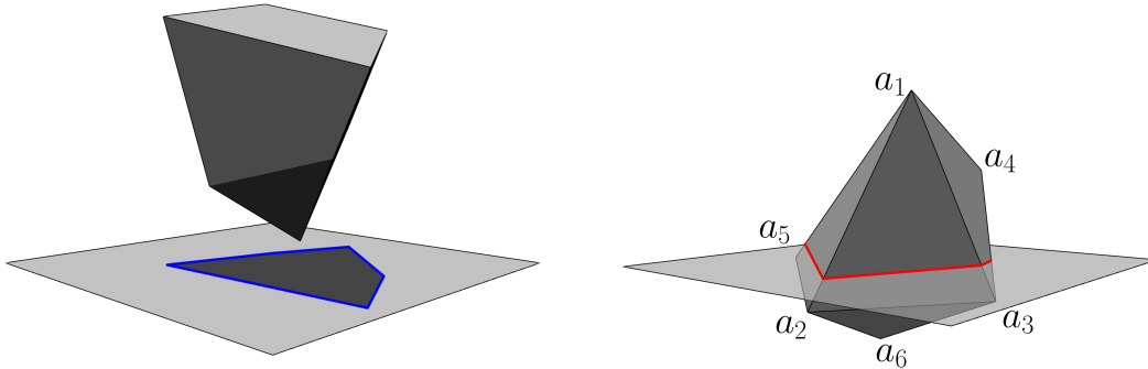
Figure 2: On the left, a polytope and its shadow. On the right, the corresponding polar polytope intersected with the plane. There are as many edges marked blue as there are edges marked red.
