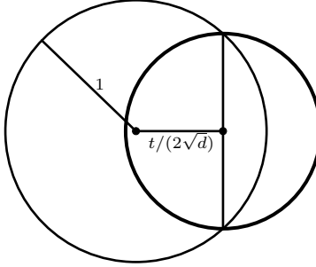
Figure 1: The small sphere has at least as much surface area as combined surface area of the enclosed sphere cap and the opposite cap together by the monotonicity of surface area (Lemma 1).
