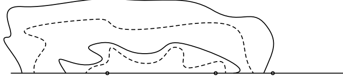
Figure 1: The event \{T(i) \geq 2\} occurs.
