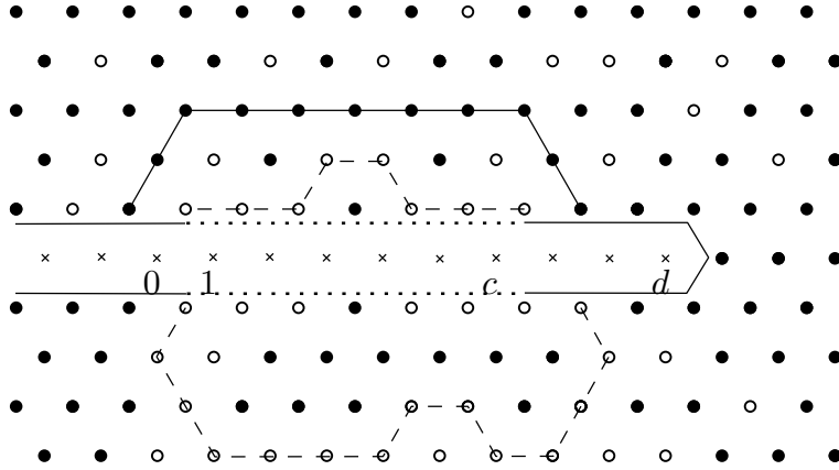
Figure 3: Illustration of the event \tilde{T}(i) = 1 ; here c = a(i), d = a(i + 1) . The half-line L(i) cut out of the lattice is indicated by x's. The boundaries \partial_{\mathbb{T}}(-\infty, 0] and \partial_{\mathbb{T}}[a(i) + 1, a(i + 1)] are indicated by solid lines and the boundary \partial_{\mathbb{T}}[1, a(i)] by dotted lines. Filled circles are open and empty circles are closed. The solid path denotes an open connection and the dashed paths denote closed connections.
