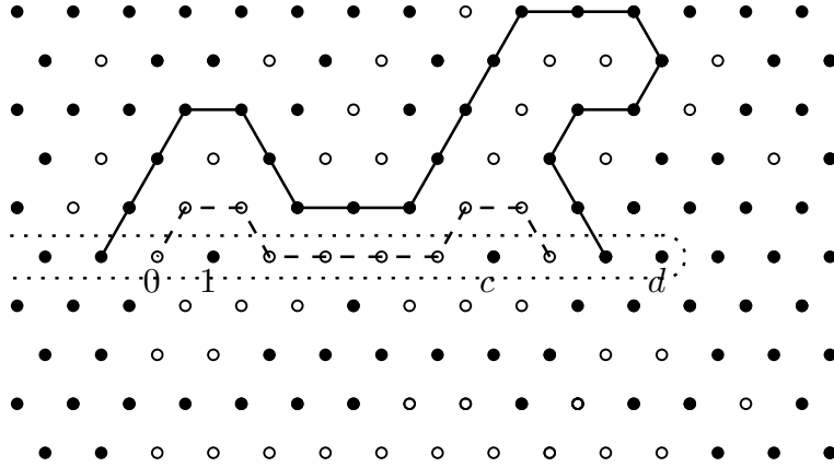
Figure 2: The event B(i) occurs. Filled circles are open and empty circles are closed. c = a(i) , d = a(i + 1) .
