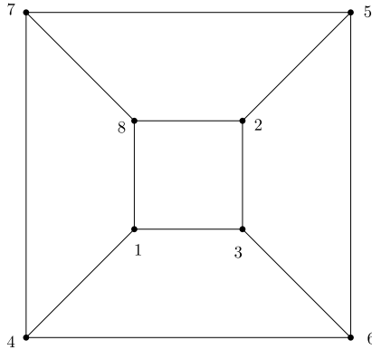
Fig. 1. The graph of Example 1.
