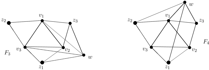
Fig. 4. The subgraphs F_3 and F_4 .
