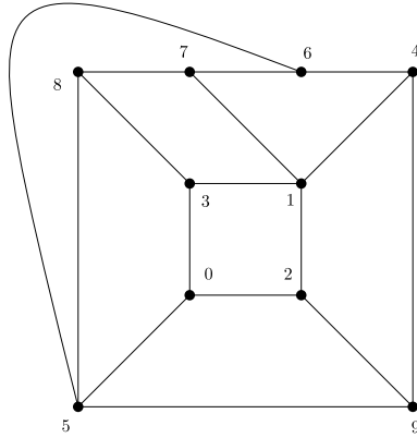
Fig. 2. The graph of Example 2.
