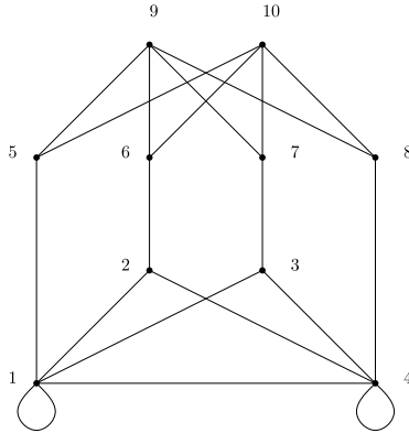
Fig. 3. The graph of Example 3.
