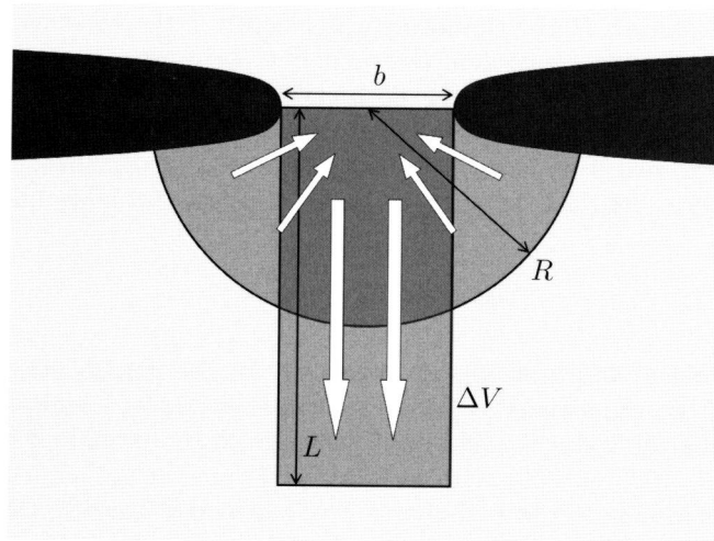
Figure 1.9: Conceptual model for the asymmetry of the flow pattern into and out of the narrow entrance of a basin according to Stommel & Farmer (1952). Due to inertia the outflow is a strong jet of width b and length L , whereas the same amount of water is drawn back radially uniform from a semicircle of radius R , leaving behind the volume \Delta V .
