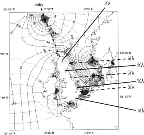
(d) The North Sea interpreted as a \frac{7}{4}\lambda -resonator
