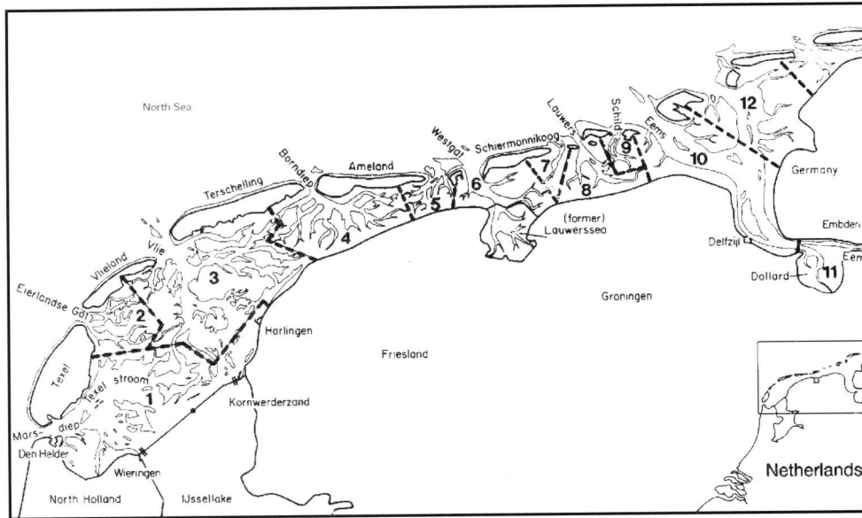
(c) Interpretation of the Dutch Wadden Sea as a number of separate Helmholtz resonators
