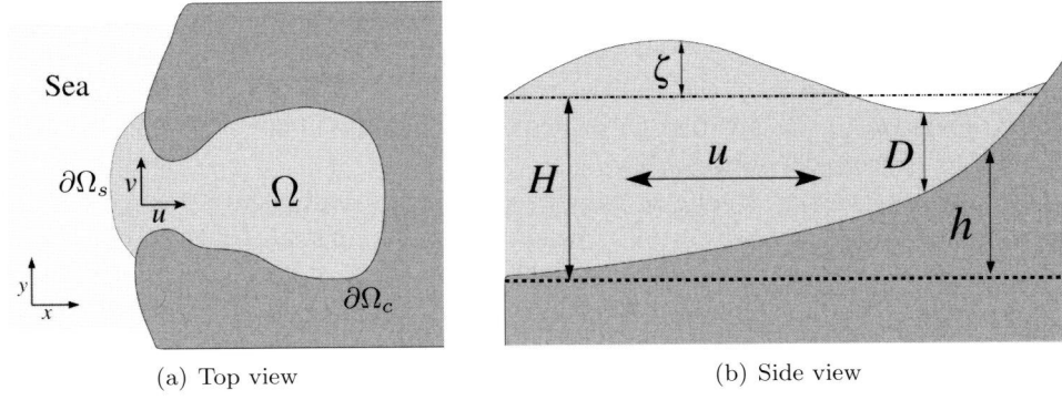
Figure 4.1: Sketch of the tidal basin.
