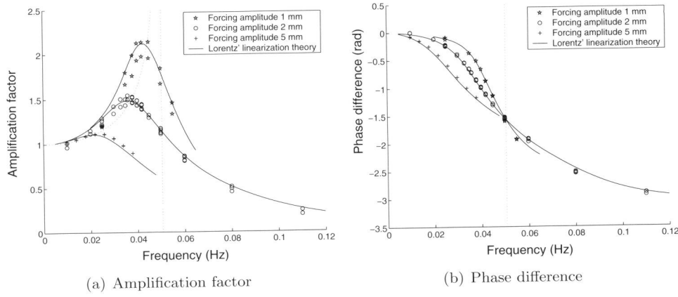
Figure 3.4: Response curves: amplification factor |\alpha|/\alpha_e and phase lag \phi between the tide at sea and in the basin as a function of forcing frequency \omega/(2\pi) . Three series of measurements with forcing amplitudes \alpha_e \approx 1, 2, 5 mm are shown, for each of which results for two sensors in the basin have been obtained. Slight amplitude differences between both basin sensors can be noted, in particular at 1 mm forcing amplitude. Solid curves show the fit to the theory (3.4). The Helmholtz frequency \omega_0 = 0.0505 Hz is indicated by a dotted vertical line, a dotted curve connects the maxima according to (3.5). Note that one fit is used to describe all three curves. Apparently the decrease of the resonator's quality is adequately described by Lorentz's linearization theory.
