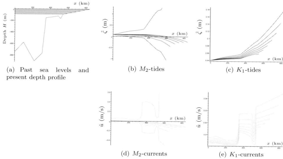
Figure 2.3: The modelled amplitude of the past tide in the Adriatic Sea when the mean sea level was lower, for the lunar semidiurnal M_2 -tide and for the diurnal K_1 -component. The results are shown for a mean sea level which is 0, 19.5, 39, 58.5, 78, 97.5 and 117 m less than present, with corresponding reduction in basin length to 840, 791, 743, 694, 645, 596 and 548 km respectively.
