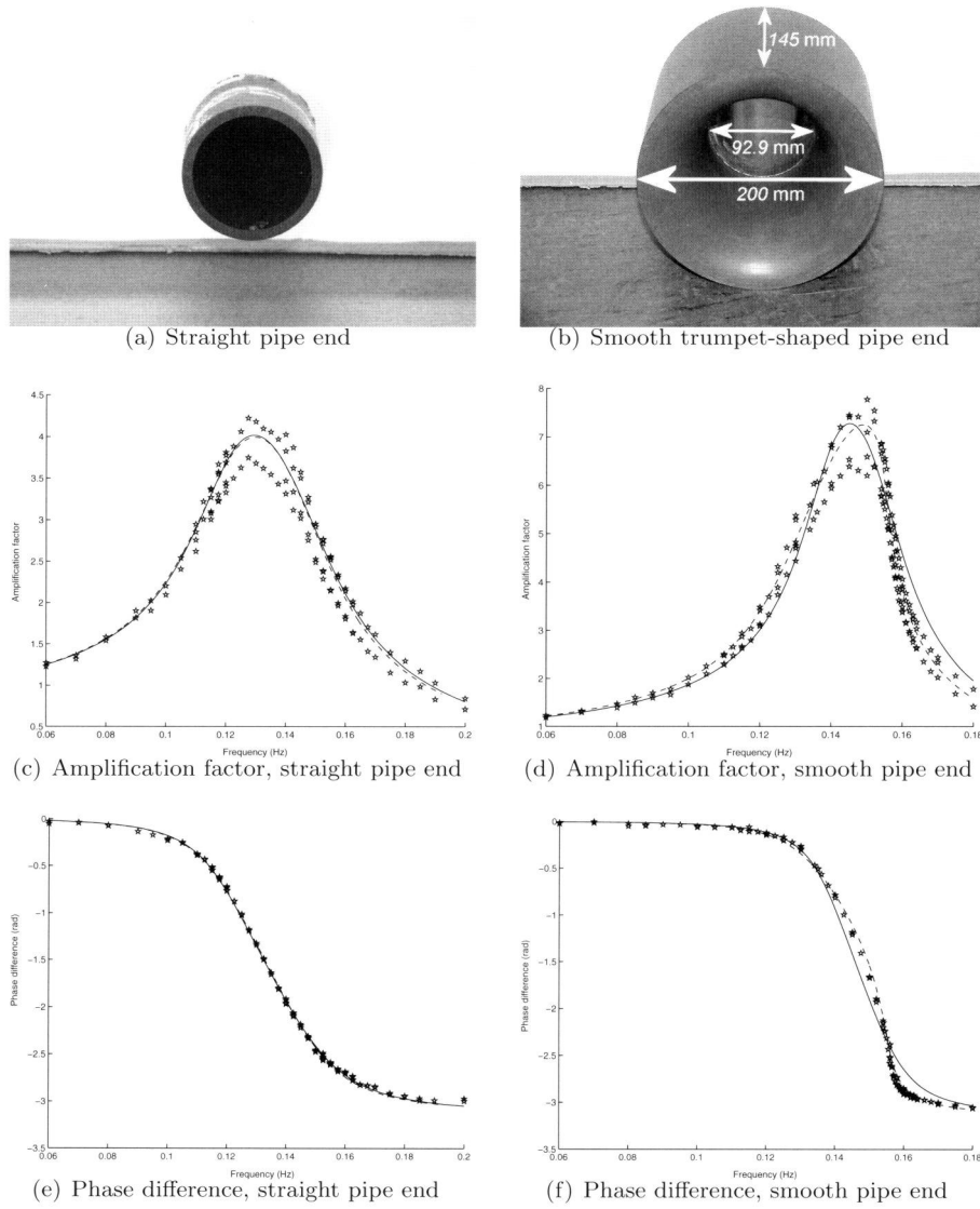
Figure 6.9: Response curves with and without smooth trumpet-shaped pipe ends. Forcing amplitude \alpha_e \approx 1 mm in both cases. The straight pipe (left) is 313 mm long with 92.9 mm inner diameter, the smooth pipe (right) has a total length of 340 mm including 145 mm trumpet-shaped openings at either side, in which the inner diameter increases from 92.9 mm at the interior to 200 mm at the ends. On the basin side, the lower part of the entrance has been cut to better merge with the basin's bottom. Solid curves show the fit to Lorentz's theory (6.4) with parameters \omega_0 = 0.134 Hz and \nu_0 = 62.2 m -1 in the straight pipe case, \omega_0 = 0.147 Hz and \nu_0 = 18.1 m -1 in the smooth entrance case. Dashed curves show the extended nonlinear theory (6.6) with parameters \omega_0 = 0.133 Hz, \nu_0 = 61.1 m -1 and \Gamma = 0.60 \cdot 10^3 m -2 in the straight pipe case, \omega_0 = 0.141 Hz, \nu_0 = 16.0 m -1 and \Gamma = 1.08 \cdot 10^3 m -2 in the smooth entrance case. Again amplitude differences within the basin can be seen between the sensors at the end and entrance of the basin respectively.
