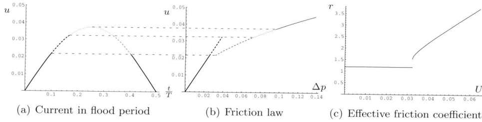
Figure 6.11: Sketch of frictional pressure difference during half a tidal period. 6.11(b) shows the friction law that was used, with a transition region between the laminar and turbulent regime. In 6.11(a) the regime of the flow at different intervals during the flood period is indicated. The effective friction coefficient determined from Lorentz's linearization procedure is shown in 6.11(c).
