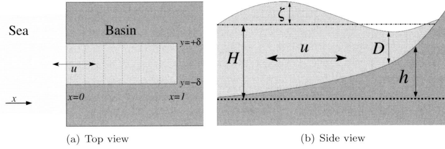
Figure 4.2: Sketch of the one-dimensional basin. Its width is much smaller than its length, the bottom profile h(x) depends on the longitudinal coordinate only, hence the motion is assumed to be restricted to the longitudinal direction.
