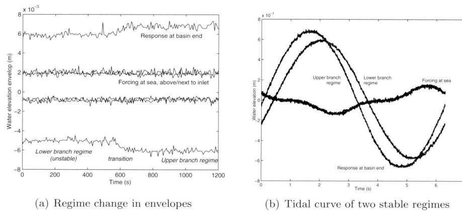
Figure 6.8: Illustrations of multiple equilibria: 6.8(a) Time series of the envelop of forcing at sea and response in the basin by plotting measurements of high and low tide. The forcing conditions remain at frequency 0.1592 Hz and amplitude 1 mm during the entire time series, but the response shifts to a higher amplitude regime. 6.8(b) Measured tidal curves of forcing at sea and two different stable response regimes under the very same forcing conditions. Forcing is at 0.1588 Hz frequency, 1 mm amplitude for both cases, but the response has a phase lag of 2.29 rad and amplitudes of 5.5–6.8 mm for the higher amplitude regime and a phase lag of 2.65 rad and amplitudes of 5.1–5.8 mm for the lower amplitude regime. Note that overtides are clearly present at sea but do not propagate into the basin.
