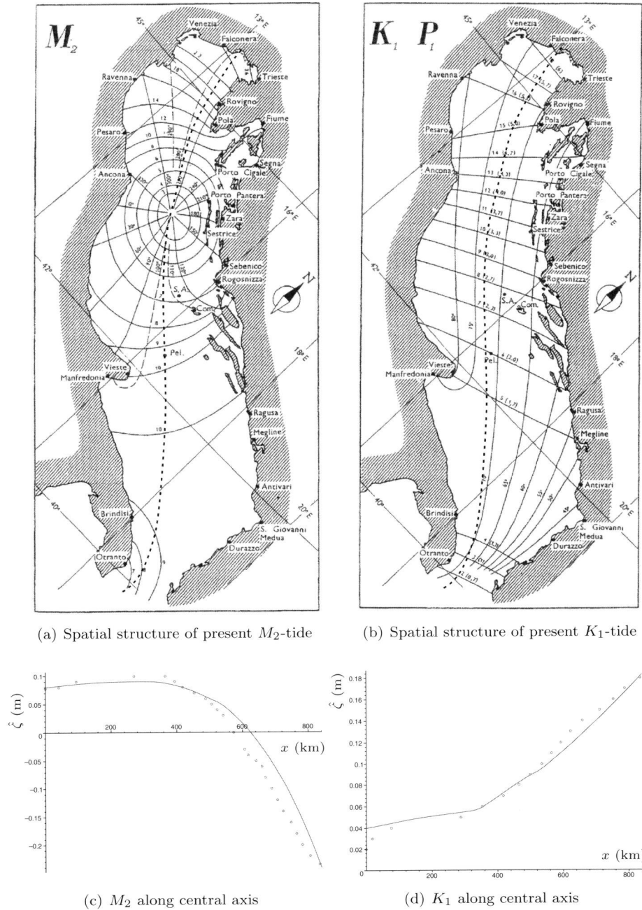
Figure 2.2: (a) and (b) show the structure of the present lunar semidiurnal M_2 ( 12^h25^m period) and the diurnal K_1 -tide ( 23^h56^m period), after Cushman-Roisin & Naimie (2002, Fig. 2) (originally Polli, 1960). The dashed curve denotes the central axis along which the values have been used for comparison with the model. (c) and (d) compare the tidal elevation amplitude (m) obtained from the one-dimensional linear model (solid line) with those from tidal observations (circles).
