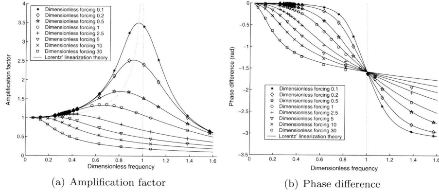
Figure 3.5: Response curves: amplification factor and phase lag between the tide at sea and in the basin as a function of forcing frequency. Numerical results (symbols) for the dimensionless system (3.7) are shown. The dimensionless Helmholtz frequency \omega'_0 = 1 is indicated by a dotted vertical line, a dotted curve connects the maxima according to (3.5). The theoretical (solid) curves are calculated from (3.4),(3.5), with \omega_0 = 1, \nu_0 = \frac{8}{3\pi} .
