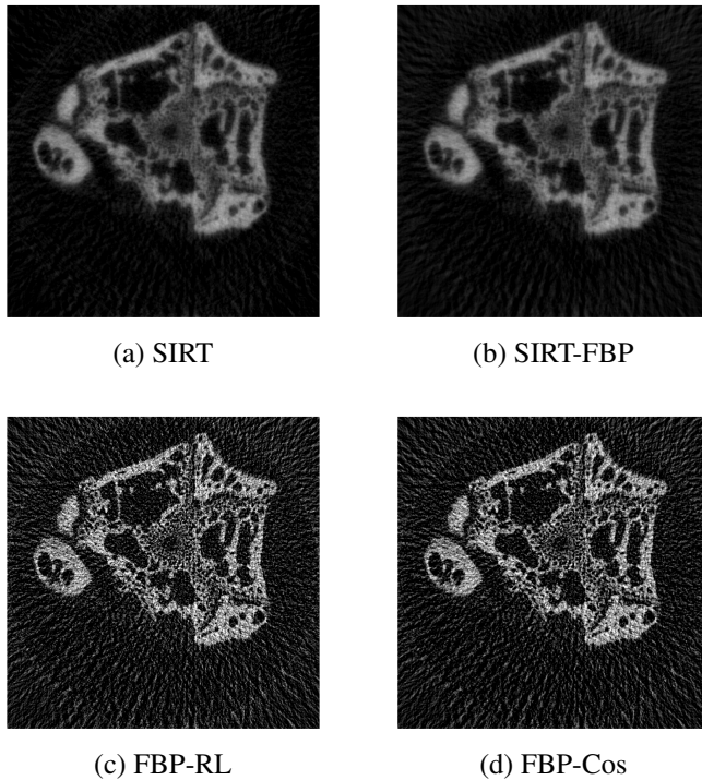
Fig. 3. Reconstructions of femur projection data with 60 projection angles and SIRT with K = 50 iterations.
