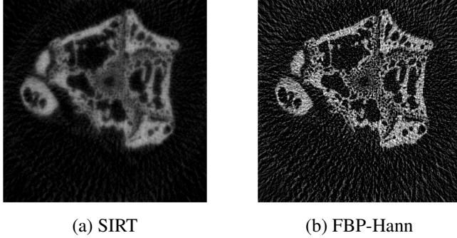
Fig. 2. Reconstructions of femur projection data with 60 projection angles and SIRT with K = 50 iterations.
