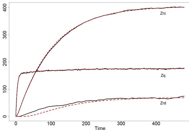
Figure 2: z_{RC}(t), z_Q(t), z_{RD}(t) (from top to bottom) via fluid limit (red dashed curve) and Z_{RC}(t), Z_Q(t), Z_{RD}(t) via simulation (black solid curve), \lambda = 40, \mu = 1/4, p = 0.5, q = 0.1, \theta = 1/2, s = 148, \delta_{RD} = 0.05, \delta_{RC} = 0.01
