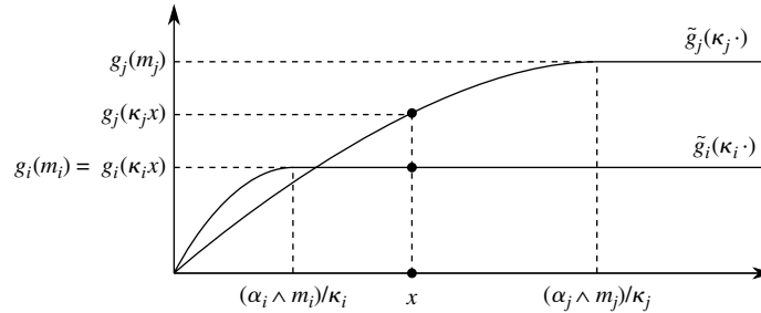
FIGURE 3. Graphs of the functions \tilde{g}_i(\cdot) ; x is the unique solution to (30).
