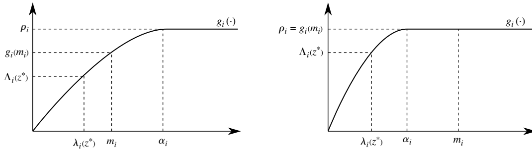
FIGURE 2. Graph of the function g_i(\cdot) in the two possible cases: when m_i \leq \alpha_i (left) and when m_i > \alpha_i (right); z^* is an invariant NFMS.
