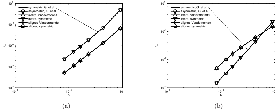
Figure 6: Error \epsilon_\infty for test cases with constant angles of misalignment, \gamma = 10 , \zeta = 10^9 , at varying mesh width, (a) \alpha = 5^\circ , (b) \alpha = 30^\circ . In the plots all symmetric schemes overlap and likewise do all asymmetric schemes
