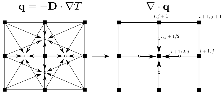
Figure 2: Asymmetric scheme, temperature T is defined on the full indices and the diffusion tensor \mathbf{D} on the half-indices
