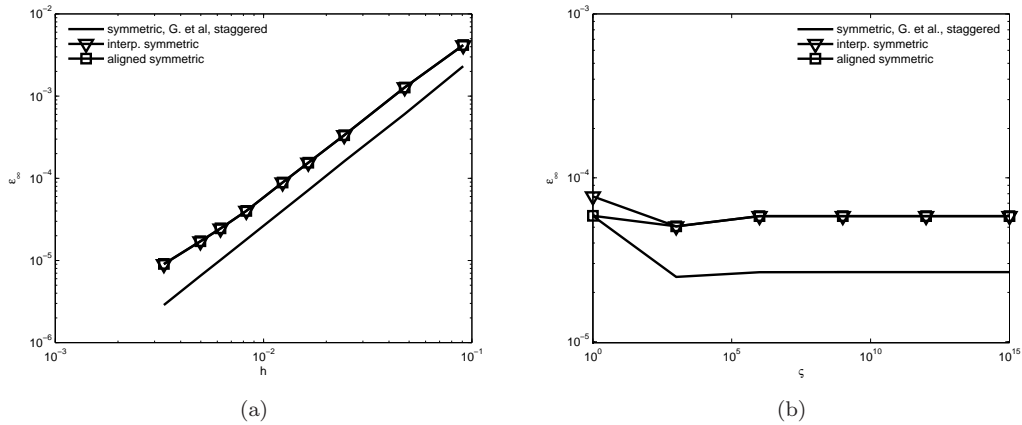
Figure 10: a = 25, b = -75 , (a) \epsilon_\infty convergence for \zeta = 10^9 , (b) \epsilon_\infty -error norm versus the anisotropy \zeta for a 100 \times 100 grid
