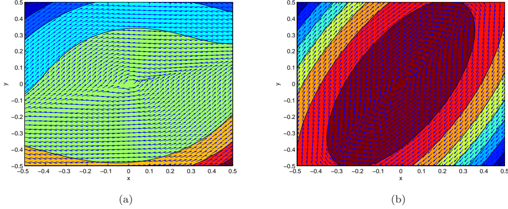
Figure 9: Tilted test cases, field line direction with (a) non-rotating field lines, a = 25, b = -75 , (b) rotating field lines, a = 0.15, b = 0.85
