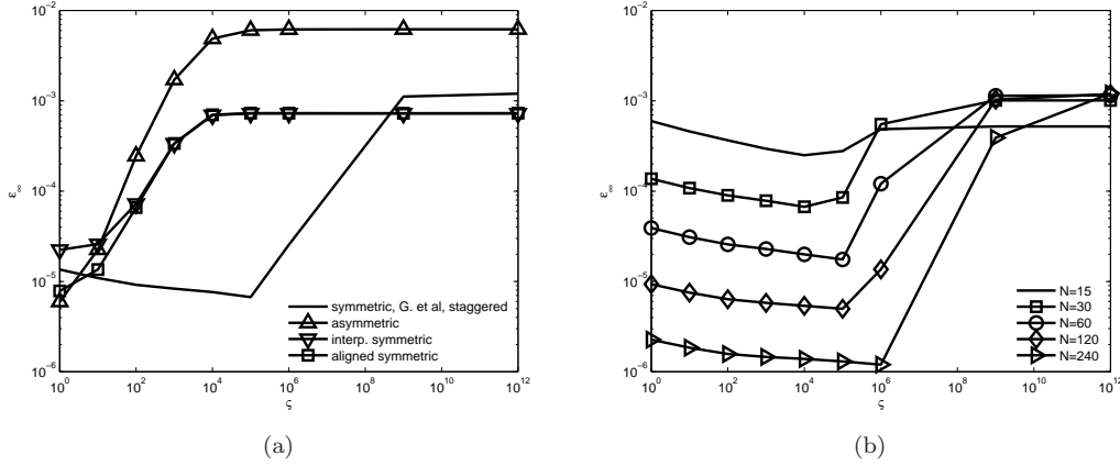
Figure 12: Second tilted test case, accuracy plot for several levels of anisotropy with a = 0.15 , b = 0.85 , \theta = \pi/3 with a grid size of 100 \times 100 , (a) aligned symmetric scheme, (b) symmetric scheme by Günter et al
