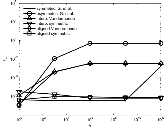
Figure 8: \epsilon_\infty -error norm versus the anisotropy \zeta for a 100 \times 100 grid
