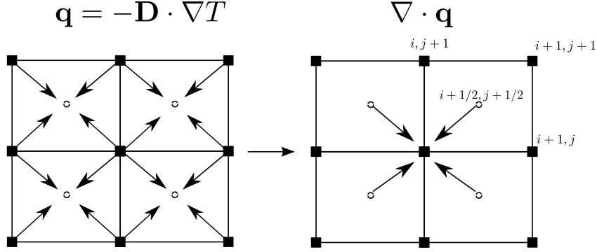
Figure 3: Symmetric scheme, temperature T is defined on the full indices and the diffusion tensor \mathbf{D} on the half-indices
