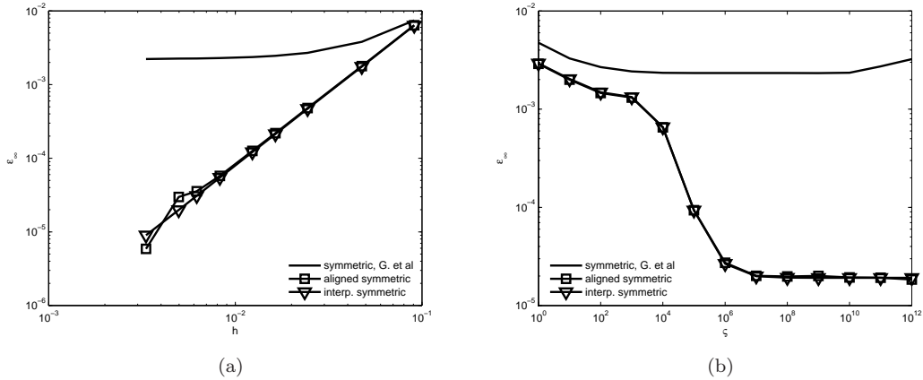
Figure 13: Test case 1 with temperature-dependent diffusion coefficients, \epsilon_\infty -error, (a) convergence for \zeta = 10^9 , (b) dependence on anisotropy for a 100 \times 100 grid
