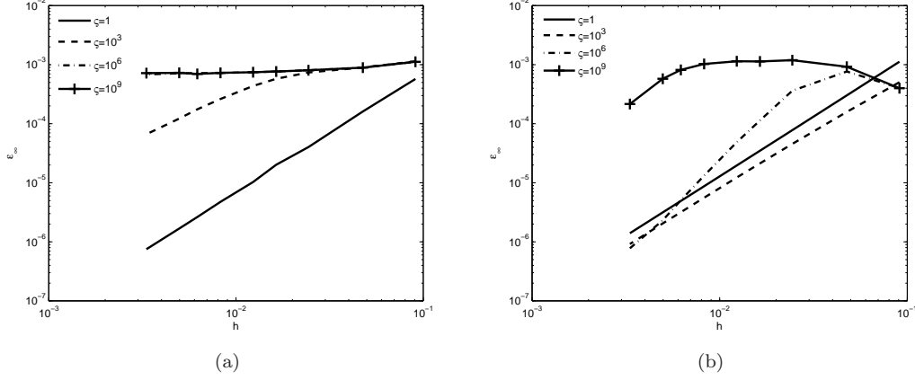
Figure 11: Second tilted test case, convergence plots for several levels of anisotropy with a = 0.15 , b = 0.85 , \theta = \pi/3 , (a) aligned symmetric scheme, (b) symmetric scheme by Günter et al
