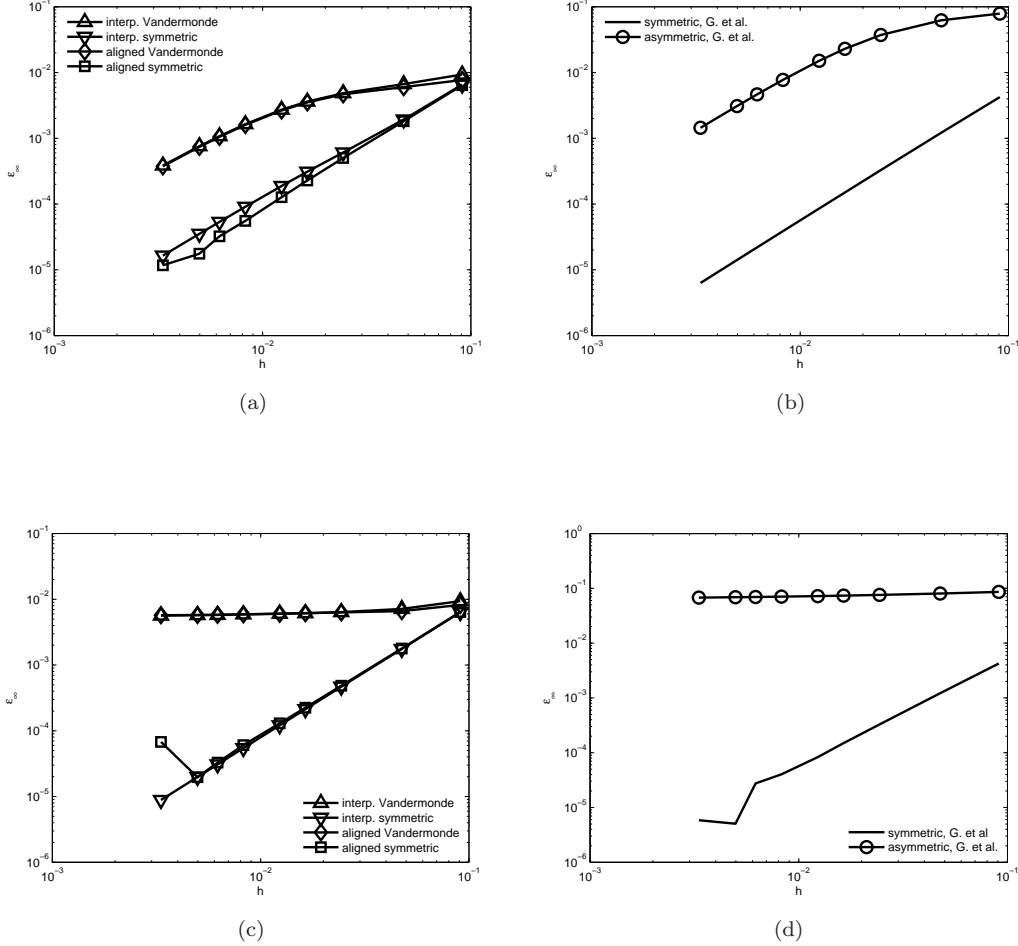
Figure 7: Error \epsilon_{\infty} for test cases with varying misalignment, (a) co-located \zeta = 10^3 , (b) staggered \zeta = 10^3 , (c) co-located \zeta = 10^9 , (d) staggered \zeta = 10^9
