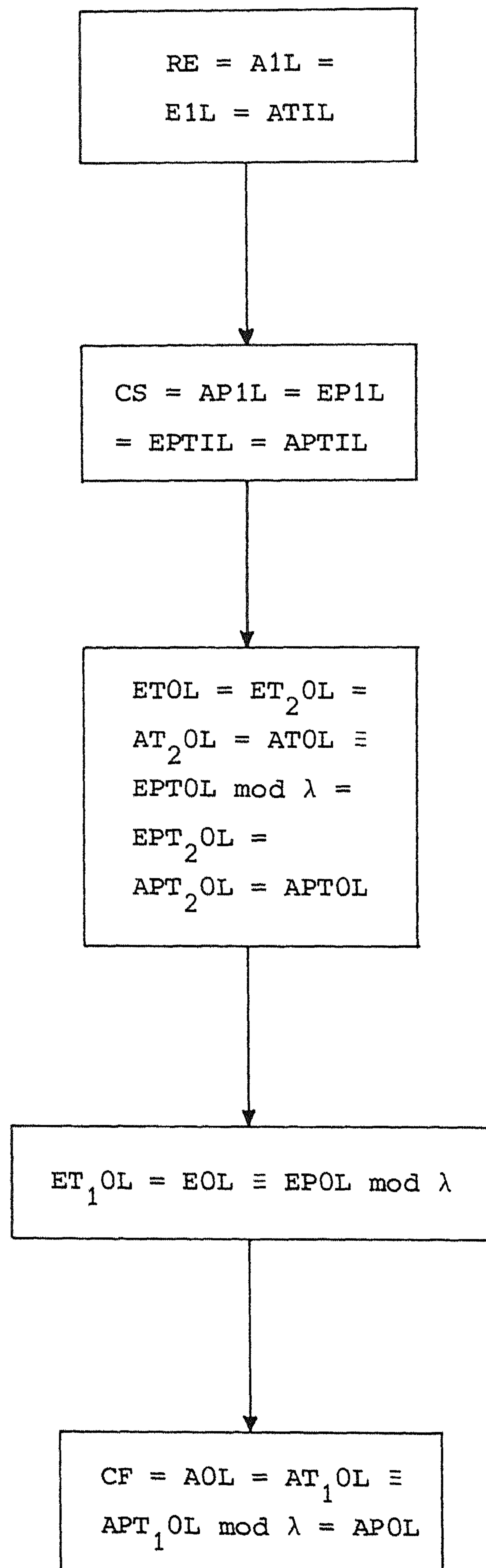
Figure 3.3. Classification of stable string language families of non-deterministic L systems with and without tables.
