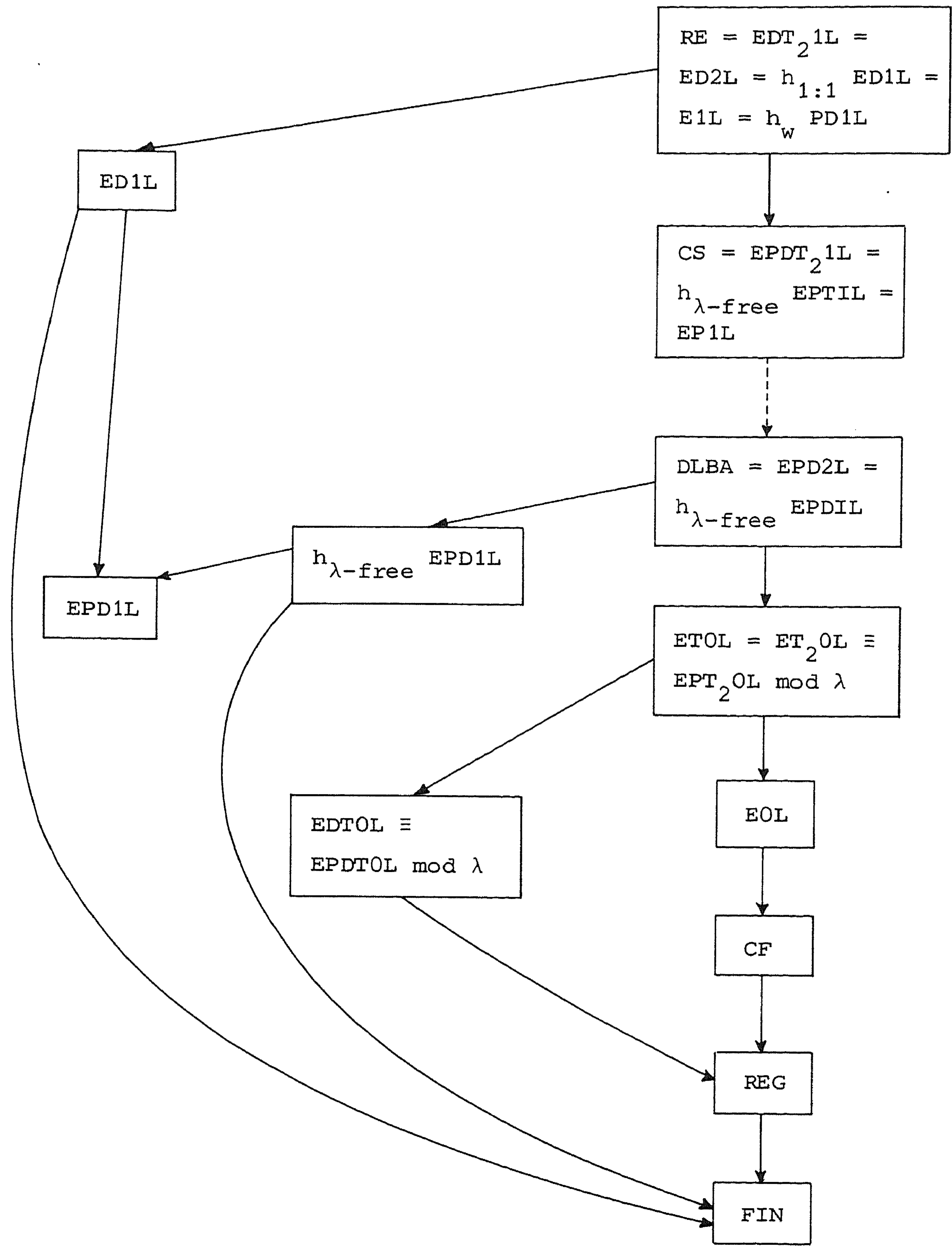
Figure 3.2. Classification of families of context sensitive table L extension languages and their homomorphic closures.
