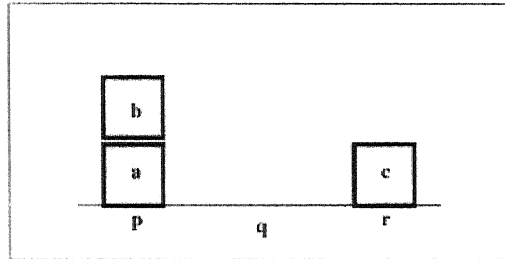
Figure 1: The Blocks-World
