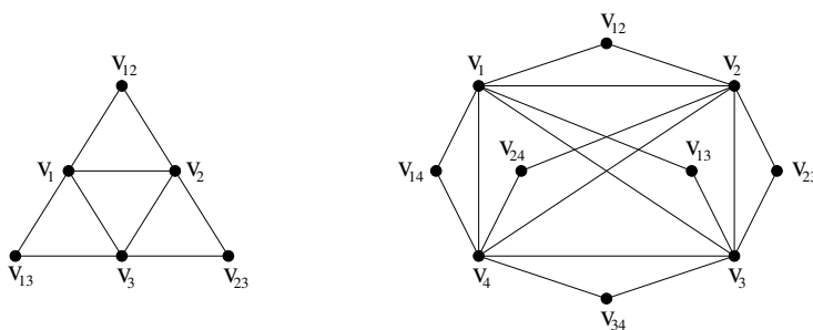
Figure 10.1: The graphs F_3 and F_4 .
