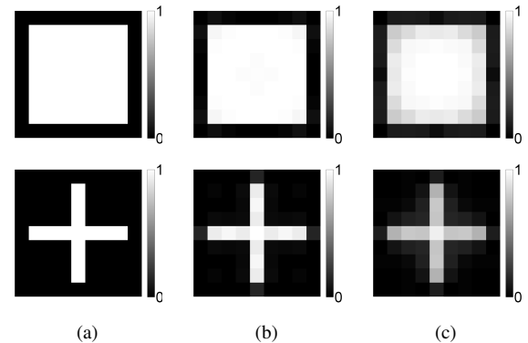
Fig. 1. Test objects and their reconstructions when placed in the center of the reconstruction region; (a) original, (b) SIRT, (c) FBP.
