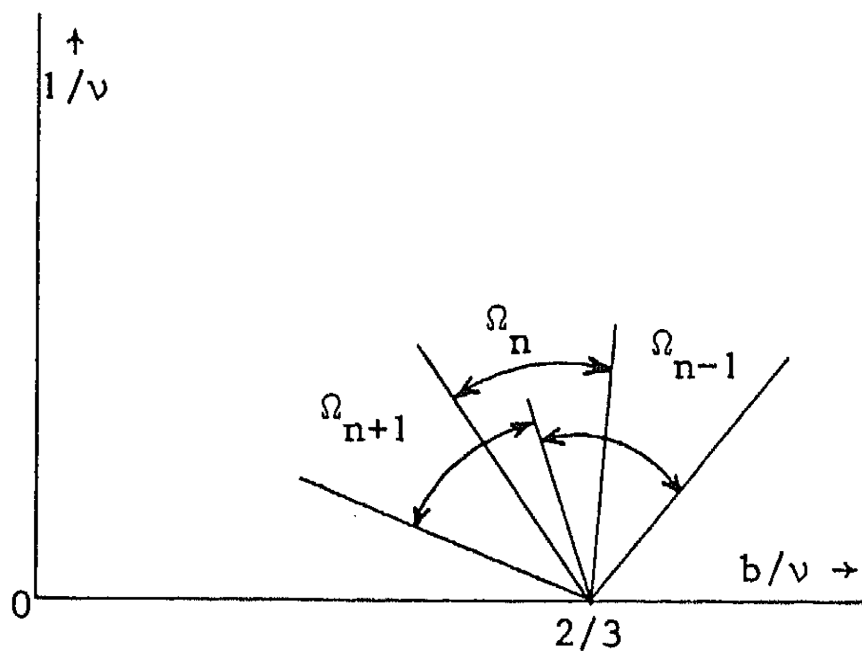
FIG. 2. Local structure of the domains \Omega_n near (b/v, 1/v) = (2/3, \infty) derived from the formal asymptotic analysis. Exact values are given in Fig. 1 (dotted lines) for n \leq 4 .
