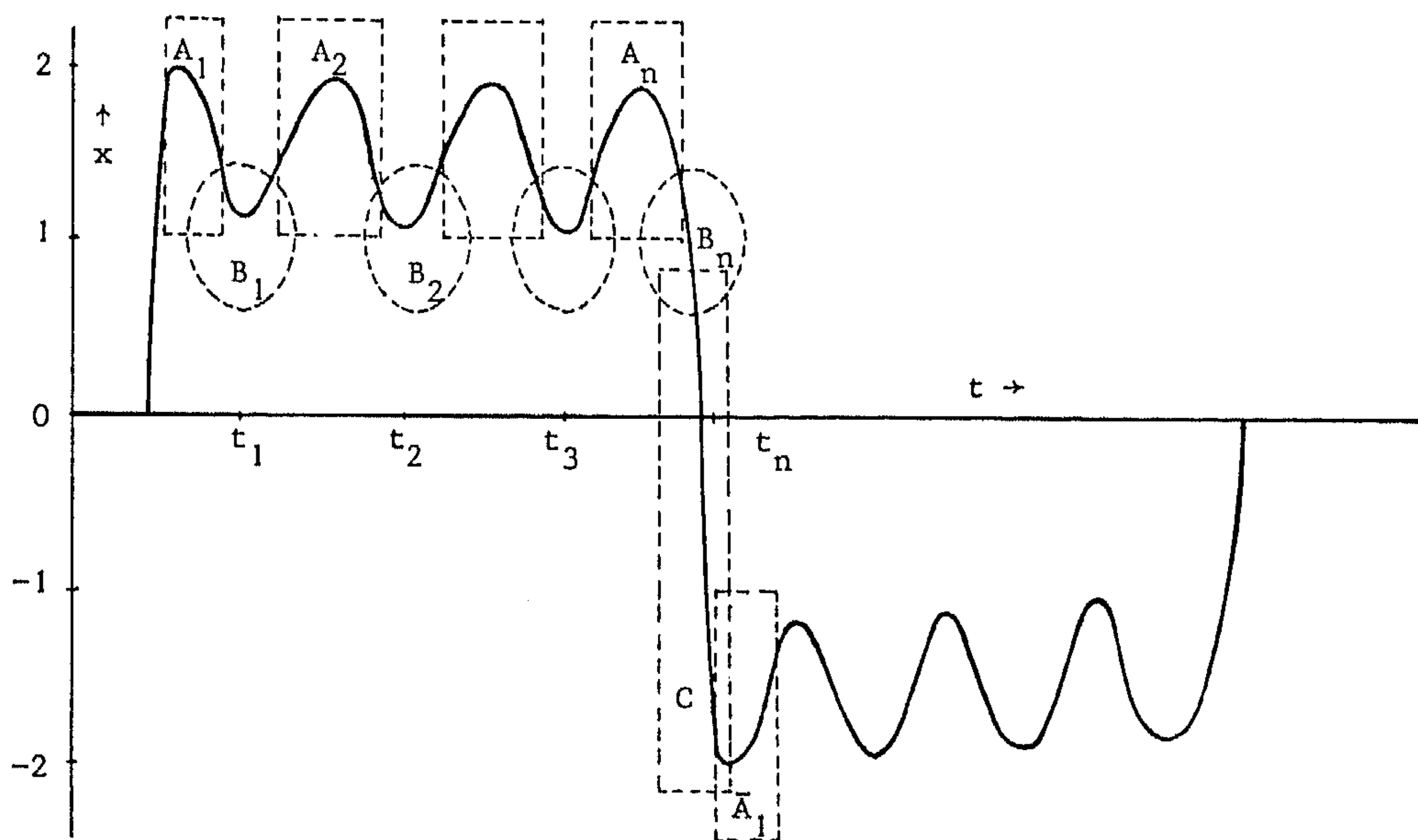
FIG. 3. Characteristic regions for a periodic solution of (1.6).
