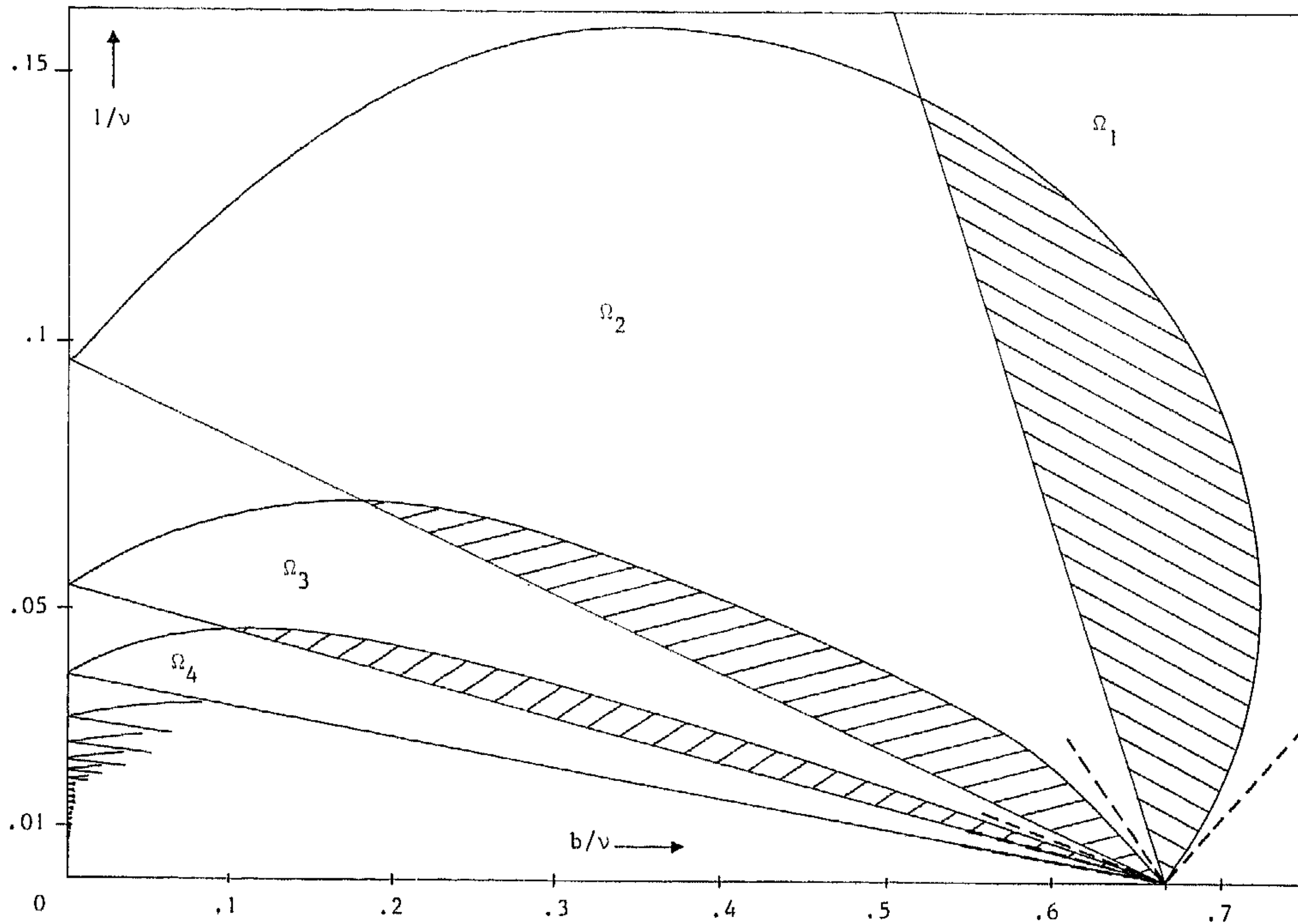
FIG. 1. The domains \Omega_n with a periodic solution T = 2\pi(2n - 1) .
