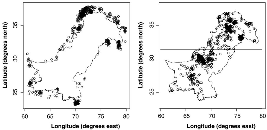
Fig. 3 Earthquake locations in ( left ) a zone up to about one degree removed from the Pakistan border and ( right ) within the Pakistan territory during the years 1973–2008. The line in the rightmost panel is at 31.4 degrees latitude
