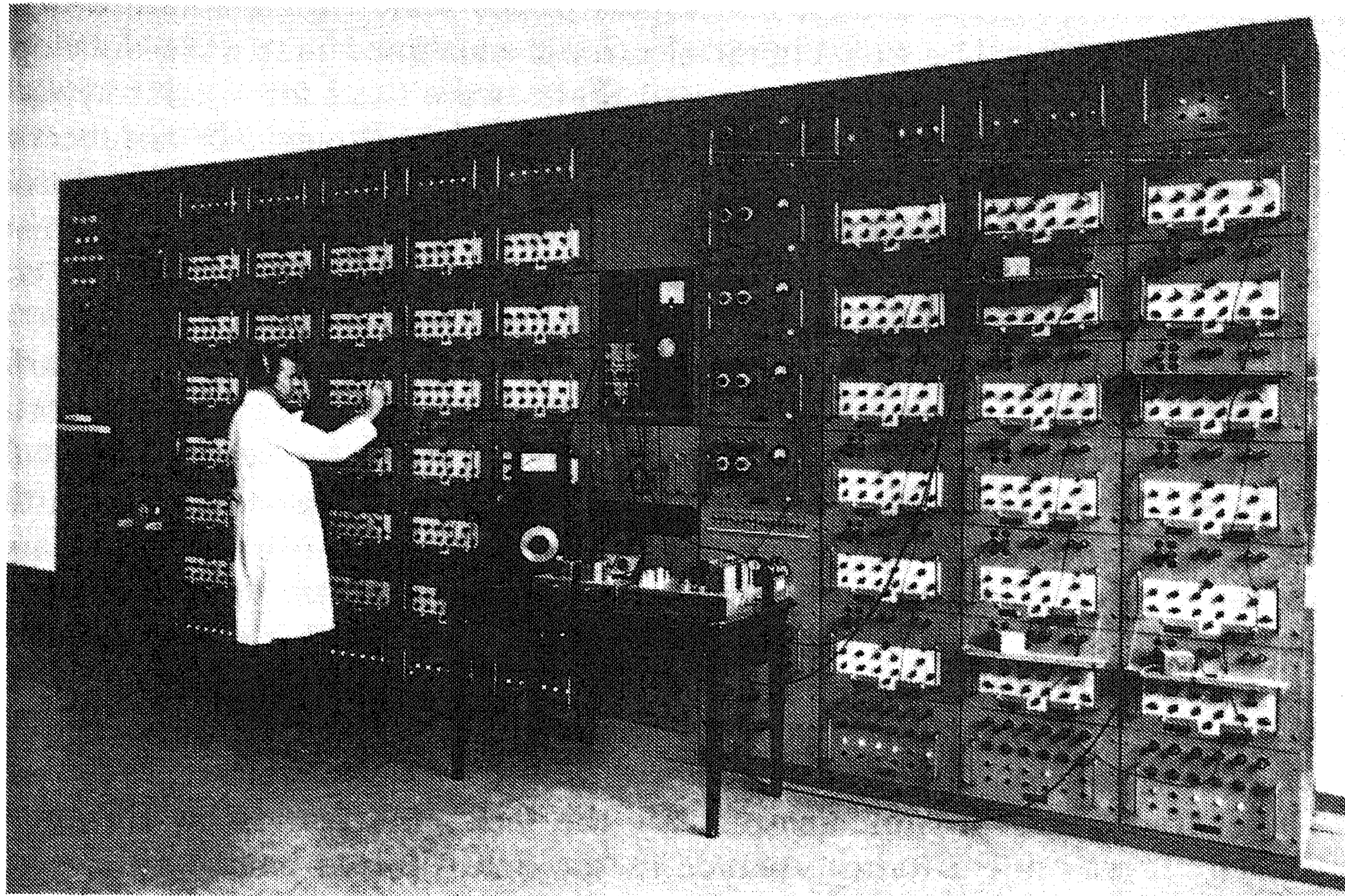
FIGURE 4. The electrical analog machine (1954). (Photo: National Public Works Administration.)
