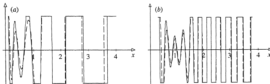
Figure 3. Numerical experiments on the approximation of theorem 4.1 for large n and x \in (0, 4] . Continuous lines represent the Laguerre polynomial L_n^{(4)}(nx) for (a) n = 10 and (b) n = 20 . Dashed lines represent the first-order approximation given by A_0\Phi_0(x, n) + B_0\Psi_0(x, n) . Both graphics are cut for extreme values of the polynomials.
