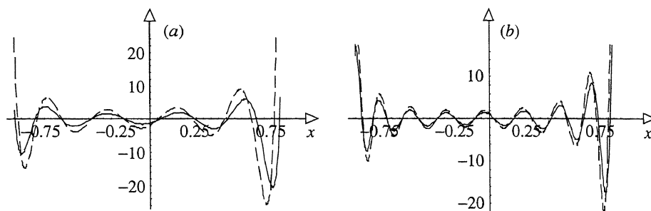
Figure 4. Numerical experiments about the approximation of theorem 5.1 for large n and -1 < x < 1 . Continuous lines represent the Jacobi polynomial P_n^{(3,4)}(x) for (a) n = 10 and (b) n = 20 . Dashed lines represent the first-order approximation given by A_0\Phi_0 + B_0\Psi_0 .
