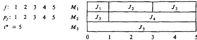
Fig. 6. Preemptive scheduling: an instance with m=3 and n=5 .
