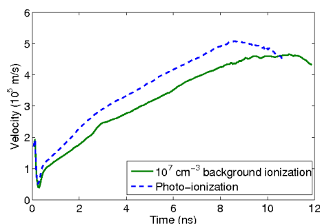
Fig. 2: Velocities of positive streamers in N_2 with a 1 ppm O_2 admixture. Simulations were done in air at 300 K and 1 bar with a 24 kV voltage over an 8 mm needle-plane gap.
