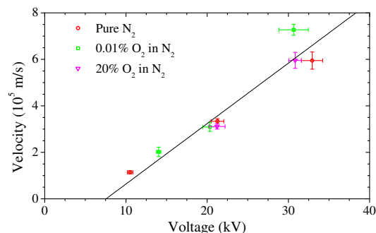
Fig. 1: Streamer velocities measured at 200 mbar for three different gasses. The horizontal error bars indicate the spread in the applied voltages, the vertical error bars indicate the sample standard deviation for 4–6 measurements. The velocities are measured roughly in the middle of the gap, except for the cases where the discharge does not reach this far (at lower voltages), in these cases, the velocity is determined at a position close to the end of the streamer channels.
