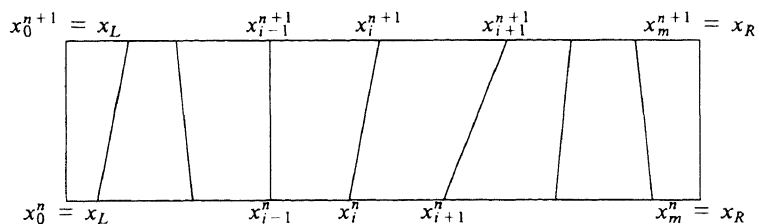
Trapezoids covering the strip x_L < x < x_R , t_n < t < t_{n+1} . (2.1)
