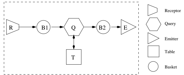
Figure 1: The DataCell model
