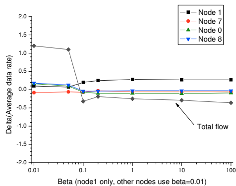
(c) Change in the average data transmission rate in comparison to global redistribution [2]
