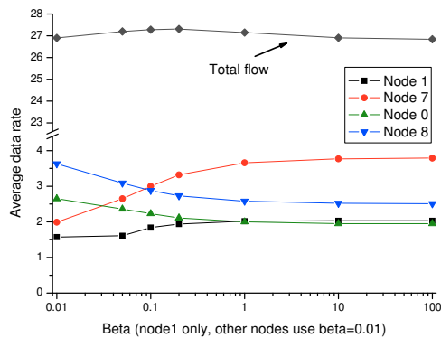
(b) Average data transmission rate
