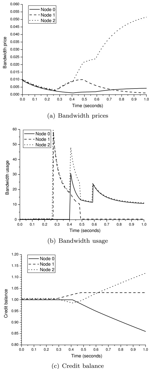
Fig. 1. The system dynamics of a 3-node network as assigned by the model derived from Crowcroft et al. [2].
