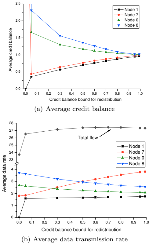
Fig. 6. Local redistribution versus the credit threshold b .
