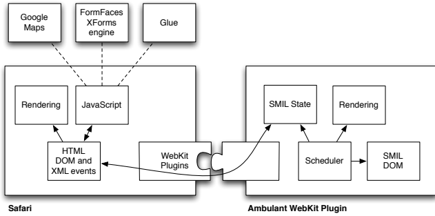
Figure 3. Browser plugin implementation
