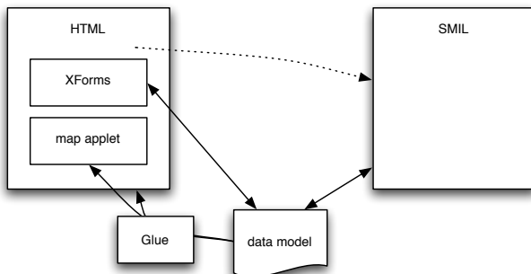
Figure 4. Guided tour document model
