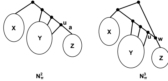
Figure 9. Networks N_\pi^2 and N_\pi^3 if Z \neq \emptyset .
