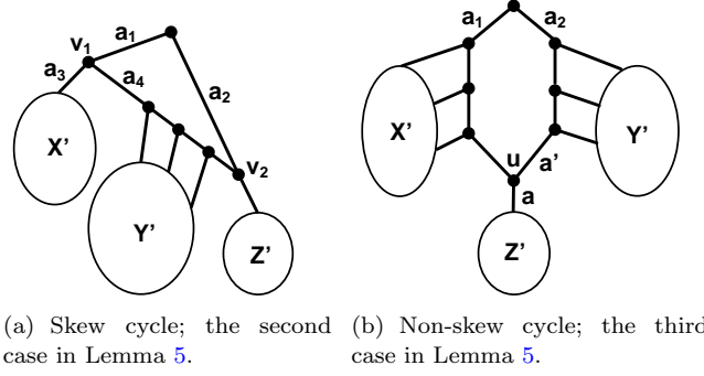
Figure 11. Shapes of networks, referred to as network N' in the proof of Lemma 5.
