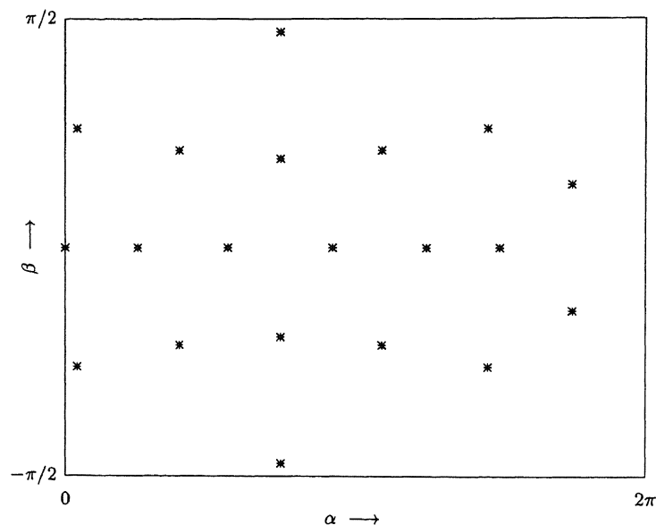
FIGURE 2. Final configuration, as in Figure 1, where the Fekete points are given in the \{\alpha, \beta\} -plane. A rotation has been applied such that (11) is fulfilled.
