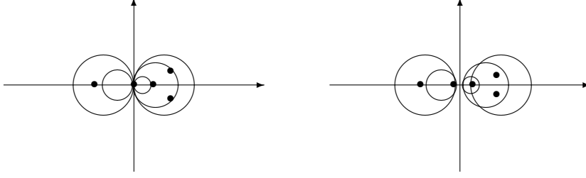
Figure 2: Eigenvalues in the complex plane. Left panel: eigenvalues of -R_A^{-1}\tilde{Q} ; right panel: eigenvalues of -R_A^{-1}(\tilde{Q} - \varepsilon D) . In this example N = 5 , and there are 3 up-states and 2 down-states.
