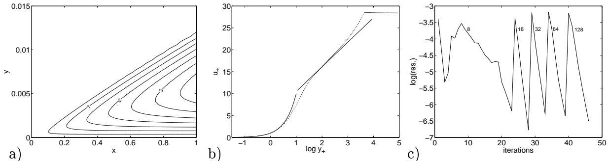
Figure 1: Turbulent flat plate flow at Re = 10^7 . Turbulent viscosity \tilde{\nu}_T \cdot 10^5 (a), velocity profile at x = 1 in wall coordinates ( \dots ) compared with analytical solution ( — ) (b) and FMG convergence (c).
