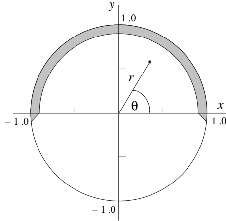
Figure 7.7. Boundary layer inside the circle along the upper boundary r = 1, y > 0 and near the points (\pm 1, 0) .
