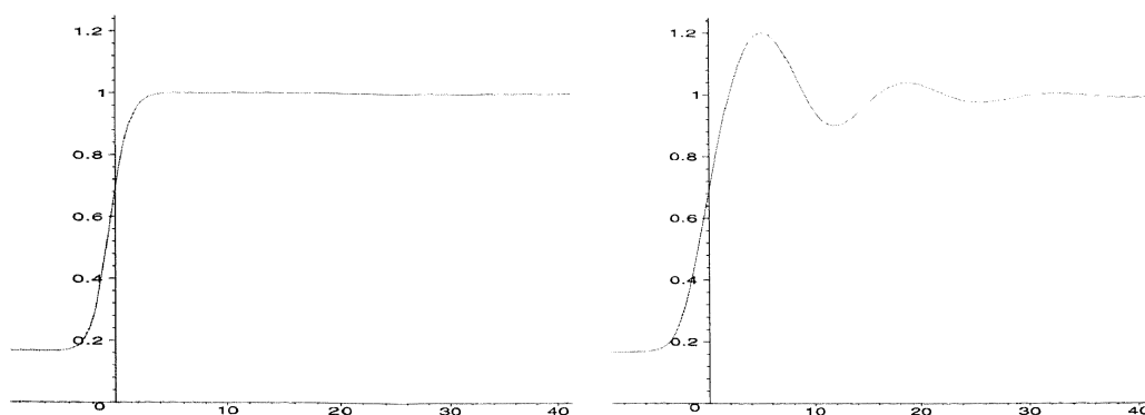
(a) Monotone profile: \varepsilon = \varepsilon^* - 0.01 \approx 0.048 .
