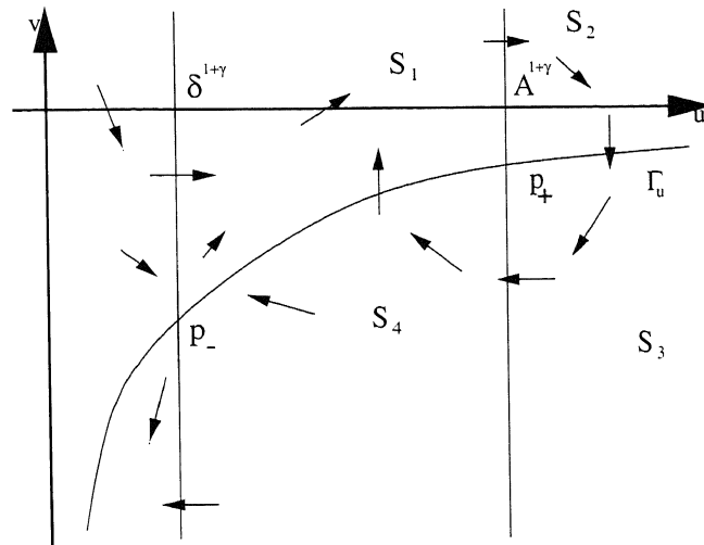
FIGURE 1. Phase plane for (P) .
