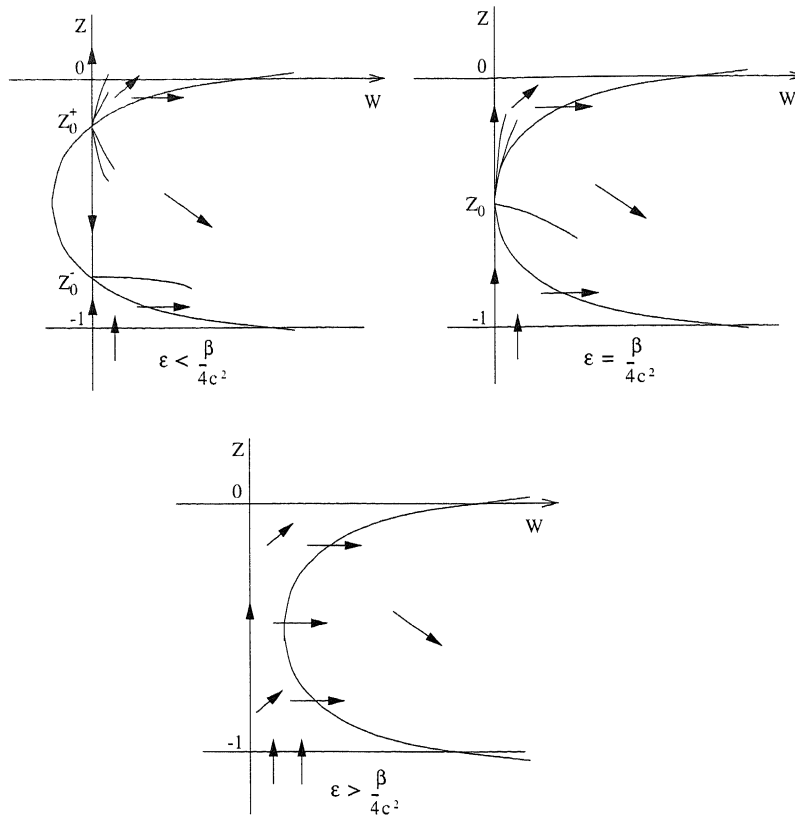
FIGURE 4. q = \frac{\beta}{1+\gamma} , 2\beta = \alpha - \gamma - 2 phase plane for different \varepsilon -values.
