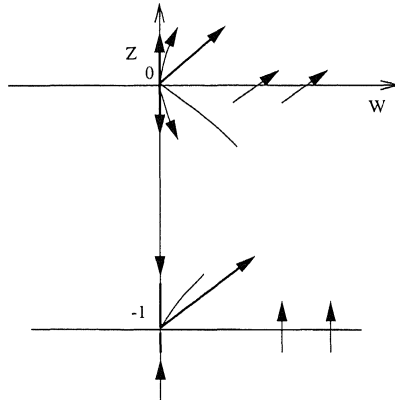
FIGURE 3. Phase plane related to (4.2), with q = \frac{\beta}{1 + \gamma} .
