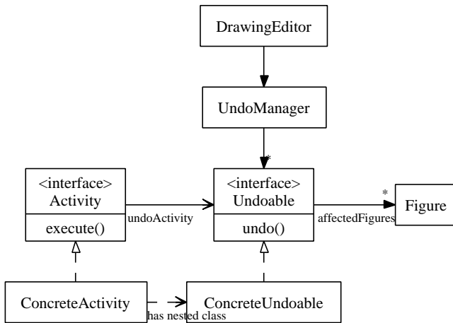
Figure 7. Participants for undo in JHOTDRAW.
