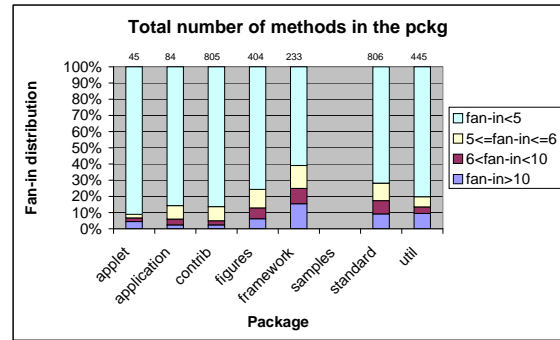
Figure 6. Fan-in statistics for JHOTDRAW.
