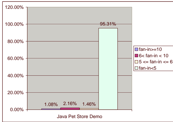
Figure 3. Fan-in distribution for PETSTORE.
