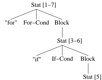
Figure 2. Source code example.
