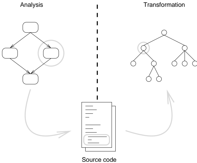
Figure 1. Source-based mappings.
