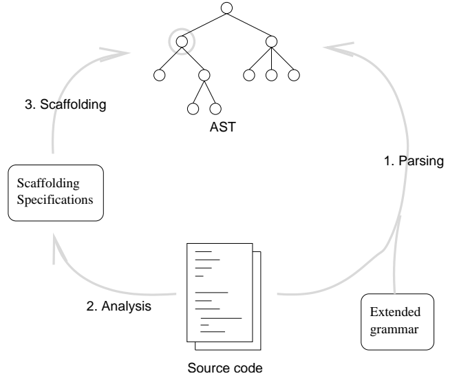
Figure 3. SCATR overview.
