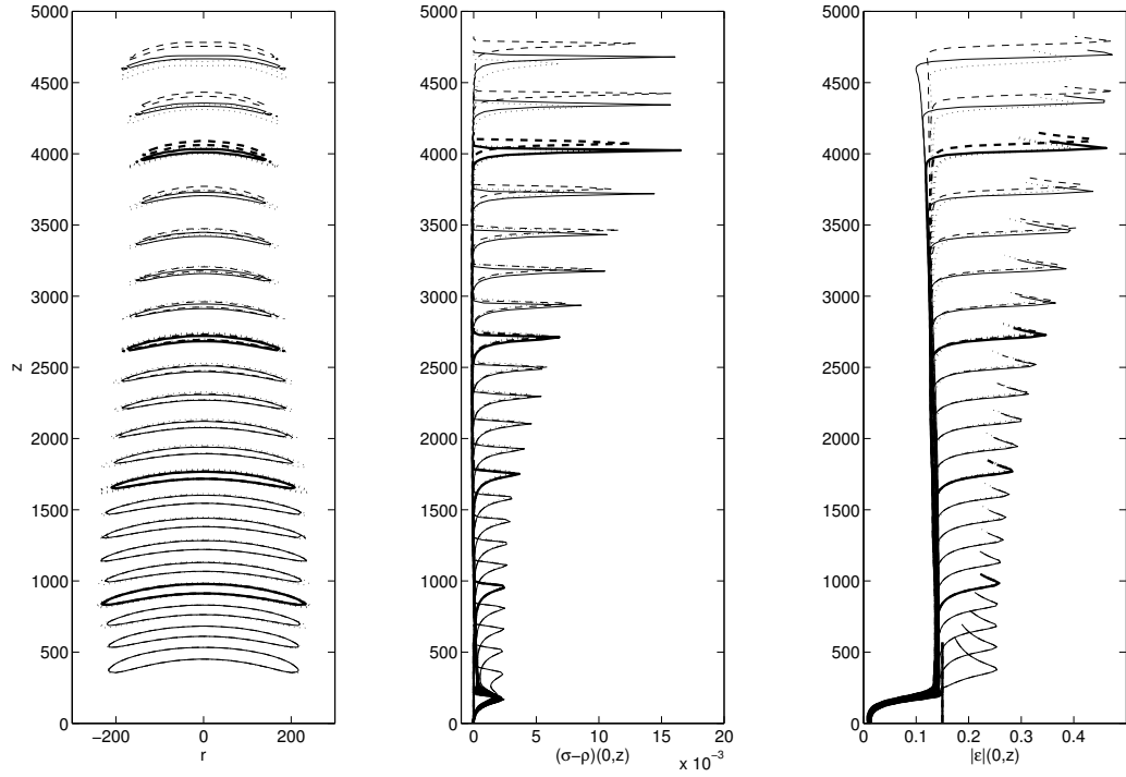
Fig. 14. Influence on the mesh size on the numerical solution for a background field of 0.15. The left panel shows the evolution of the half maximum contours of the net charge density \sigma - \rho . To show the structure clearly, the aspect ratio is not equal. The middle and the right panels show the evolution of the net charge density and the electric field strength on the axis, respectively. The times shown go from 500 to 11000 with equidistant time steps of 500. The thick lines correspond to the times shown in Fig. 13. Solid line: h_f=2 ; dashed line: h_f=4 ; dotted line: h_f=8 .
