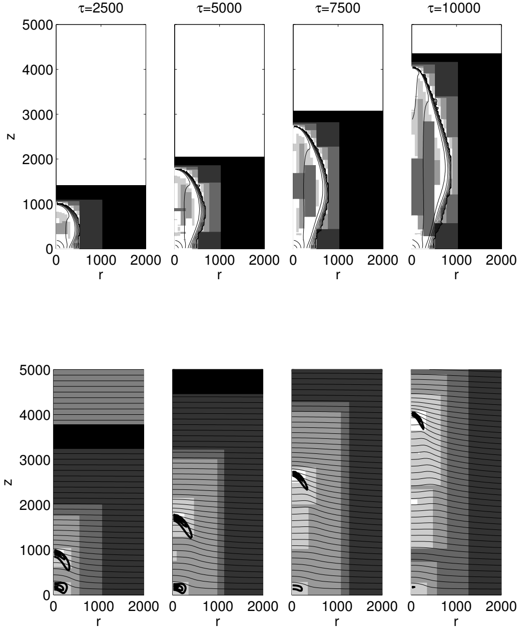
Fig. 13. Evolution of a streamer and the computational grids in a low background electric field |\mathcal{E}_b| = 0.15 . Upper panel: logarithm of the electron density with the grids for the continuity equations. The coarsest grid with mesh size 64, covering the domain on which the continuum approximation for the densities holds, is filled in black. The finest grids with mesh size 2 are white. The particle densities in the white region ahead of the streamer are below the continuum threshold and therefore not solved. Lower panel: net charge density (thick lines) and equipotential lines (thin lines) together with the grids for the Poisson equation. The white domains are covered with the finest mesh size of 2, the black regions are covered by a grid with mesh size 64. The gray region ahead of the streamer at \tau=2500 is covered by a grid with mesh size 128. The coarser grids (with mesh sizes up to 8192) are not shown.
