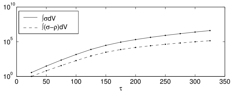
Fig. 11. Evolution of the total number of electrons (solid line) and net charge (dashed line). The lines correspond to a uniform grid computation without cutting off the densities below the continuum threshold, the dots to the refined grid computation.
