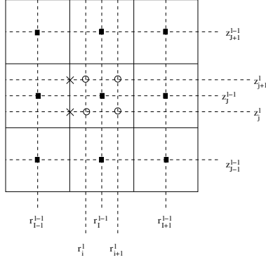
Fig. 4. The nine-points stencil used to map coarse grid values of the electric potential \phi_{IJ}^{l-1} onto the fine grid, thus obtaining \phi_{i,j}^l , \phi_{i+1,j}^l , \phi_{i,j+1}^l and \phi_{i+1,j+1}^l . The cell centers of the coarse grid are marked with ■, those of the fine grids with ○, and the boundary points of the fine grids are marked with ×.
