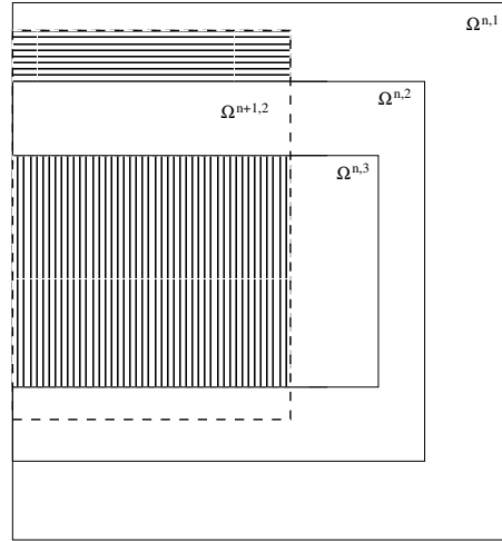
Fig. 3. Three grids at time \tau^n (solid lines) and a grid at next time step \tau^{n+1} (enclosed by the dashed lines) with the same level as \mathcal{H}^{n,2} . In the vertically striped region the new grid coincides with a finer grid at the previous time step, in the horizontally striped region only a coarser grid existed at \tau^n , and in the region that is not filled a grid at the same level existed at \tau^n .
