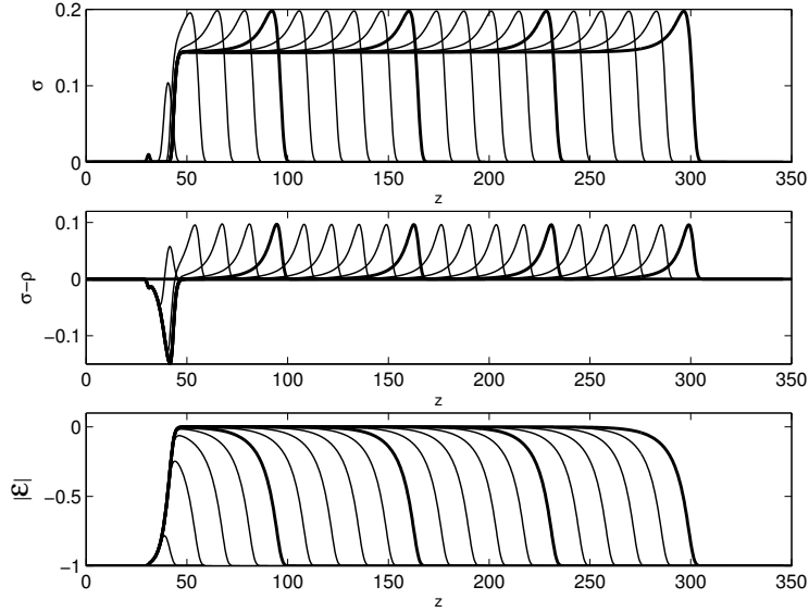
Fig. 5. Uniform grid solutions of the planar streamer front with |\mathcal{E}_b| = 1 and D = 0.1 for 0 \leq \tau \leq 200 with time steps of 10. The thick lines correspond to multiples of 50 for \tau .
