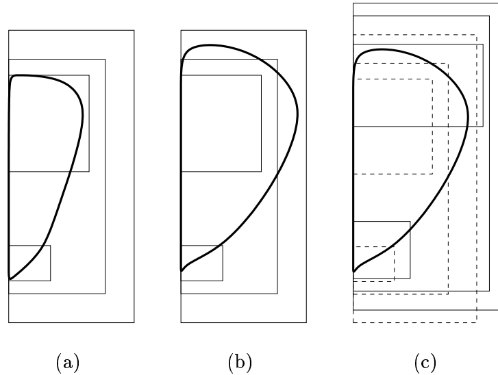
Fig. 2. (a): Contour line of the solution and the set of rectangular computational grids, both at \tau^n . (b): Contour line of the solution at \tau^{n+1} and computational grids at \tau^n . (c): Contour line and computational grids at \tau^{n+1} , the dashed lines are the grids at \tau^n .
