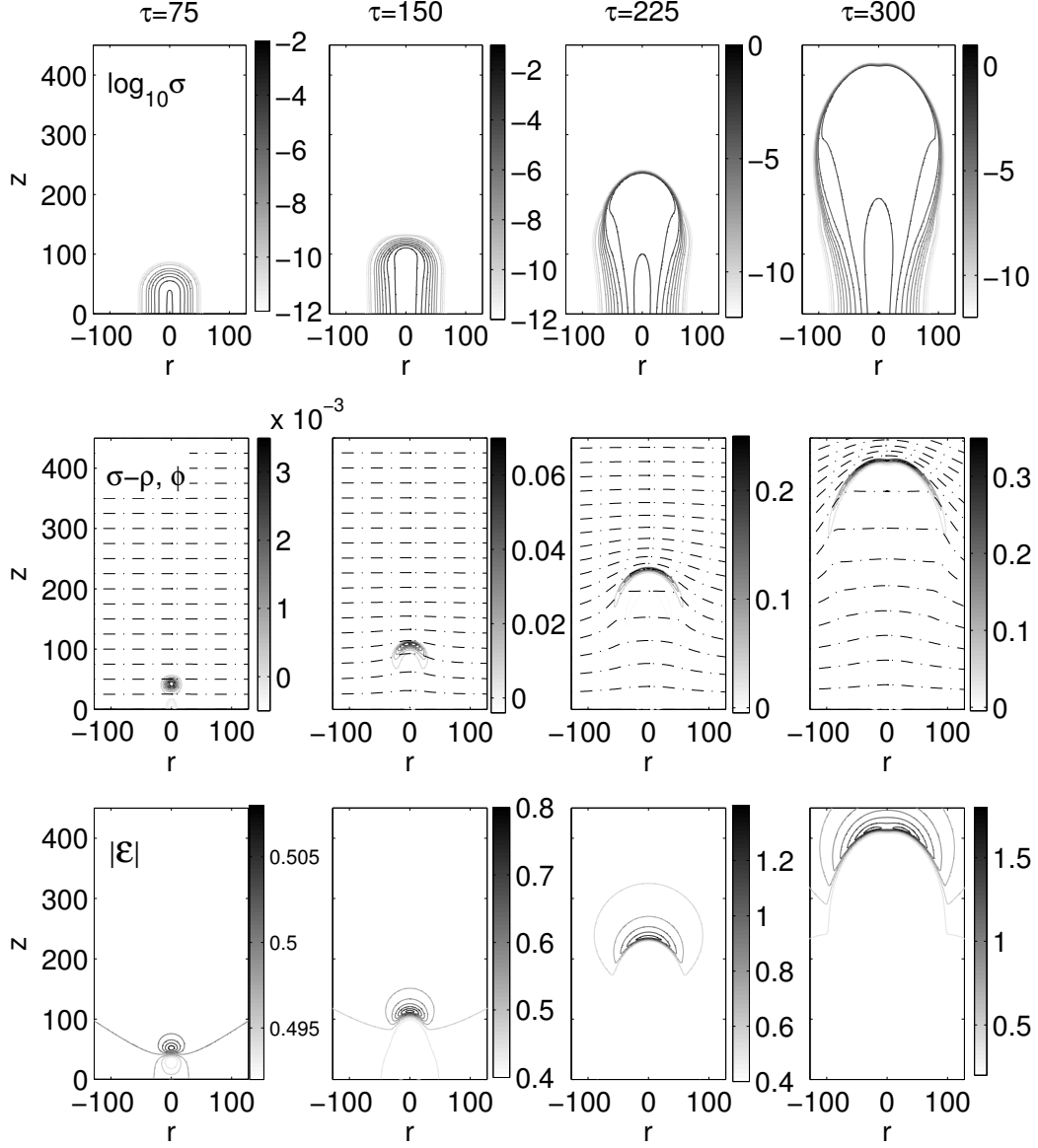
Fig. 8. Propagation of a Gaussian ionization seed as given by Eq.(6.1) in a background field |\mathcal{E}_b| = 0.5 . The snapshots correspond to times \tau=75, 150, 225 and 300 . The upper row gives the logarithm of the electron density \sigma , the middle row the net charge density \sigma - \rho and the lower figure the electric field strength |\mathcal{E}| . A uniform grid \Delta r = \Delta z = 1 has been used for both the continuity equations and the Poisson equation.
