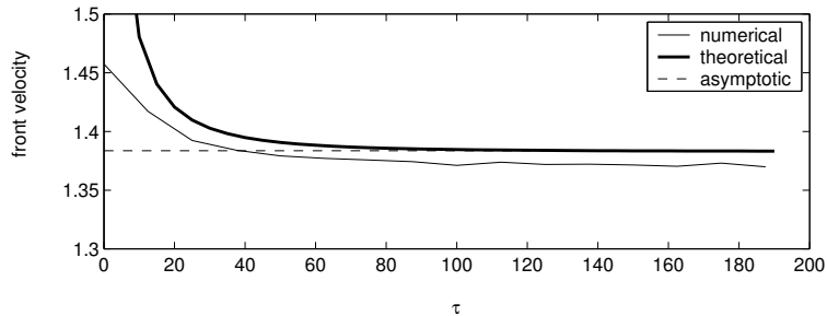
Fig. 6. Numerical front velocity (solid line) as a function of time, compared to the theoretical asymptotic front velocity v^* = 1.3863
