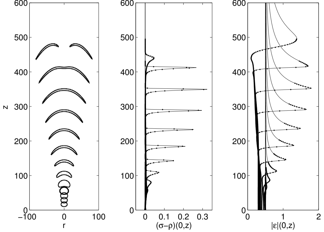
Fig. 10. Comparison of uniform grid results with those obtained using the grid refinement strategy. Left panel: evolution of the half maximum contours of the net charge density. Middle panel: evolution of the net charge density on the axis of symmetry, (\sigma - \rho)(0, z, \tau) . Right panel: evolution of the electric field strength on the axis of symmetry, |\mathcal{E}|(0, z, \tau) . The results in all panels are shown for \tau = 25 to 325, with steps of 25. Solid line: uniform grid ( \Delta r = \Delta z = 1 ), dots: grid refinement ( \Delta r = \Delta z = 1, 2 ).
