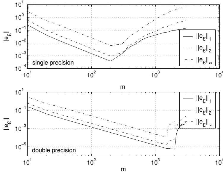
Fig. A.2. The L_1 -errors (solid), L_2 -errors (dashed) and L_\infty -errors (dash-dotted) for |\mathcal{E}| in Eq. (A.1) on m \times m grids, as a function of m . Upper panel, single precision; lower panel, double precision.
