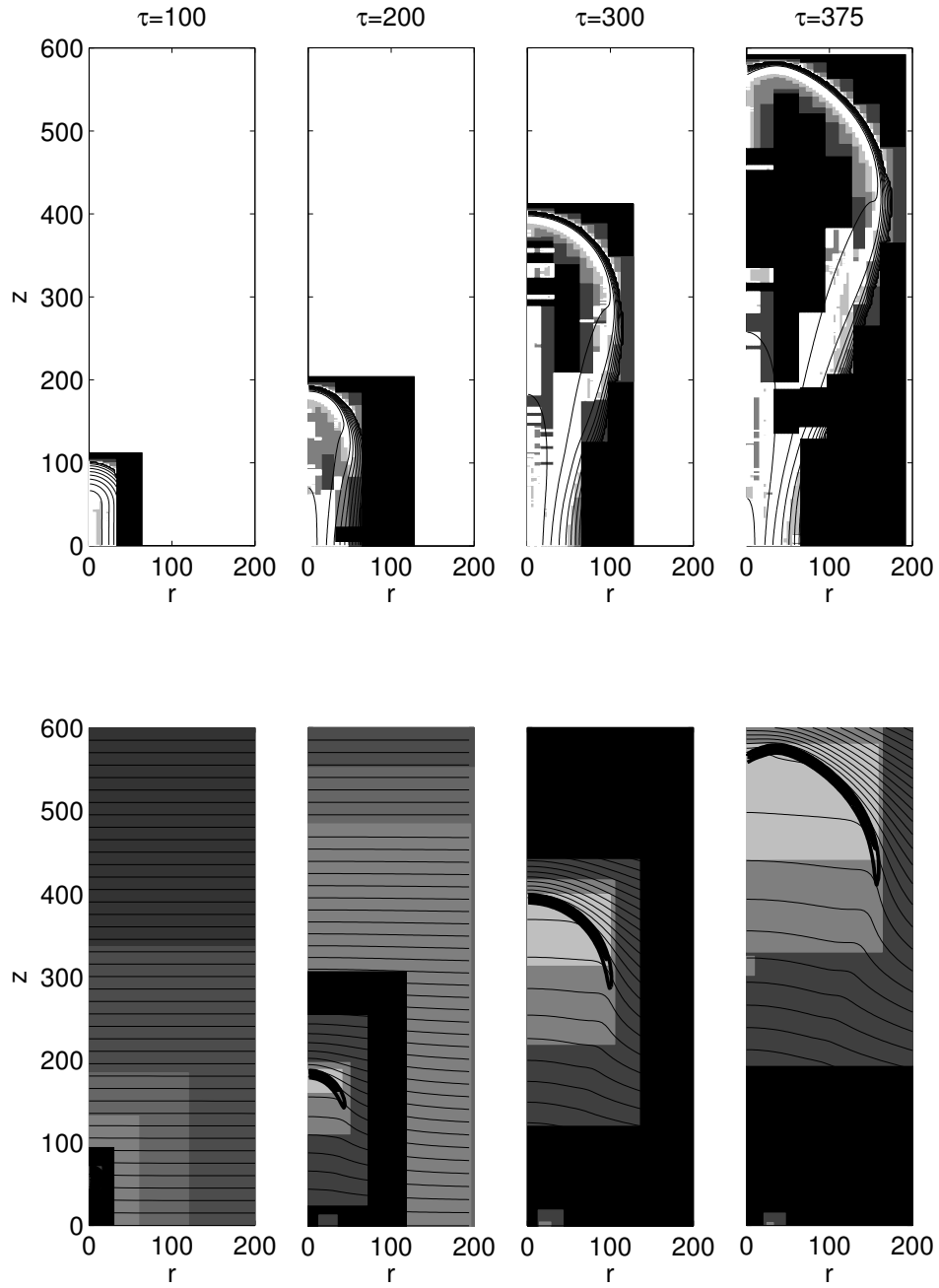
Fig. 16. Evolution of a streamer and the computational grids in a high background electric field |\mathcal{E}_b| = 0.5 . Upper panel: logarithm of the electron density together with the grids for the continuity equations. the coarsest grid has a mesh size of 2 and is filled in black. The finest grid has a mesh size of 1/8 and is white. The white region surrounding the coarsest grid has not been covered by a computational grid since the densities are below the continuum threshold there. Lower panel: net charge density (thick lines) and equipotential lines (thin lines) together with the grids for the Poisson equation. The black region is covered with a grid with mesh size 2, and the grids are refined up to a mesh of 1/8. However, this finest grid is only used at \tau=375 , in a very small part of the computational domain. The finest grid for the Poisson equation at \tau=100 has a mesh size of 1. At \tau=200 and 300 the finest grid has a mesh size of 1/4.
