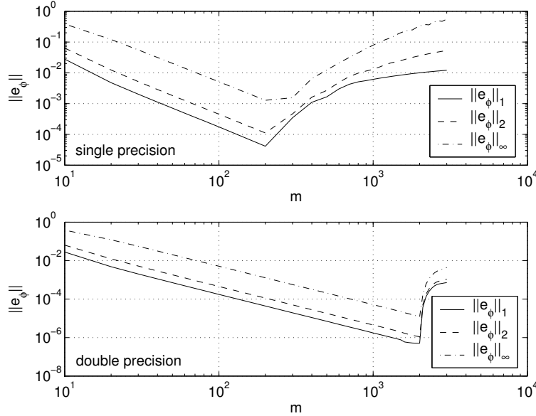
Fig. A.1. The L_1 -errors (solid), L_2 -errors (dashed) and L_\infty -errors (dash-dotted) for \phi in (A.1) on m \times m grids, as a function of m . Upper panel, single precision; lower panel, double precision.
