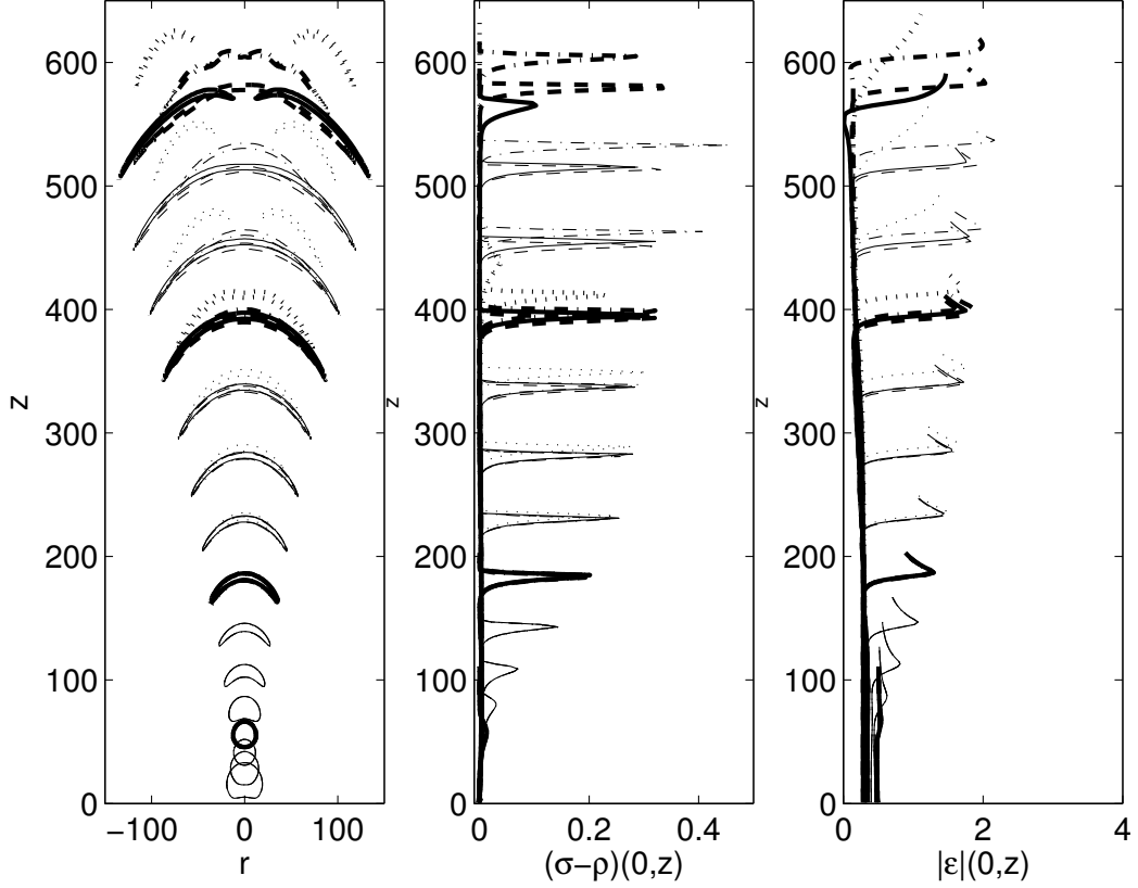
Fig. 17. Influence on the mesh size on the numerical solution for a background field of 0.15. The left panel shows the evolution of the half maximum contours of the net charge density \sigma - \rho . The middle and the right panels show the evolution of the net charge density and the electric field strength on the axis, respectively. The times shown go from 25 to 375 with equidistant time steps of 25. The thick lines correspond to the times shown in Fig. 13. Solid line: h_f = 1/8 ; dashed line: h_f = 1/4 ; dash-dotted line: h_f = 1/2 , dotted line: h_f = 1 .
