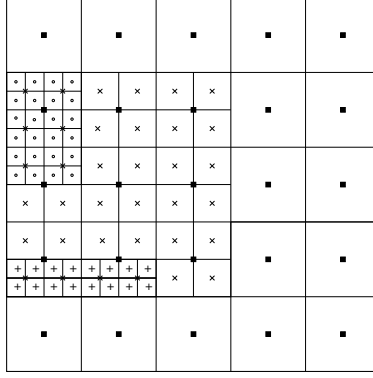
Fig. 1. An example of nested grids: ■ cell centers on \Omega^1 with l(1) = 1 , × cell centers on \Omega^2 with l(2) = 2 , + cell centers on \Omega^3 with l(3) = 3 , o cell centers on \Omega^4 with l(4) = 3 .
