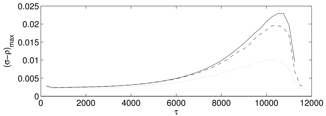
Fig. 15. Temporal evolution of the maximal net charge density on the axis. Solid line: h_f=2 ; dashed line: h_f=4 ; dotted line: h_f=8 .
