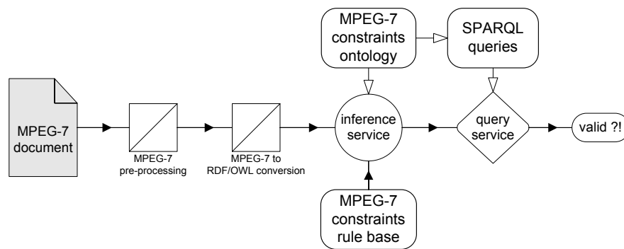
Fig. 5. Components and dataflow of the DAVP semantic validation application
