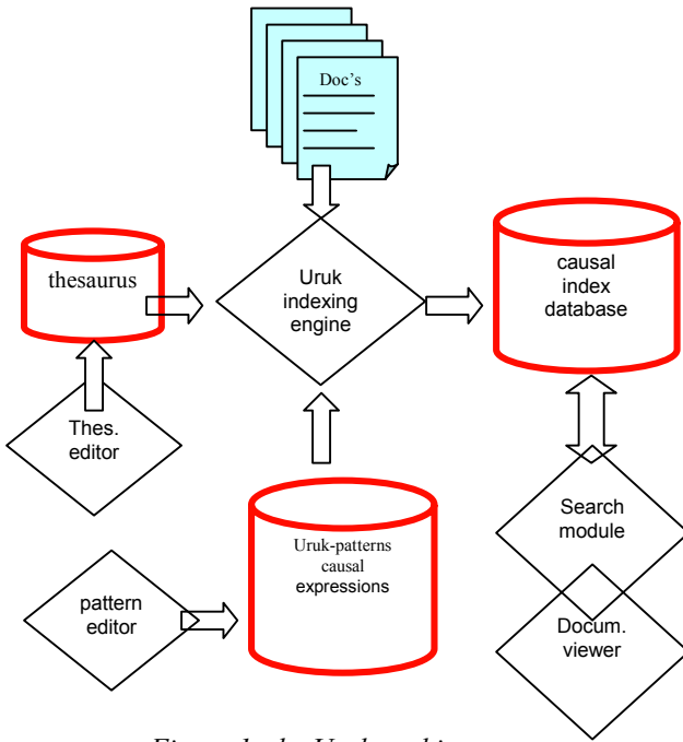
Figure 1: the Uruk-architecture
