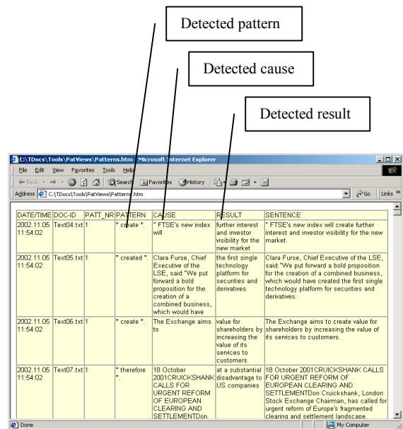
Figure 4 : screendump of PatViews which presents the detected causal patterns for a given set of documents
