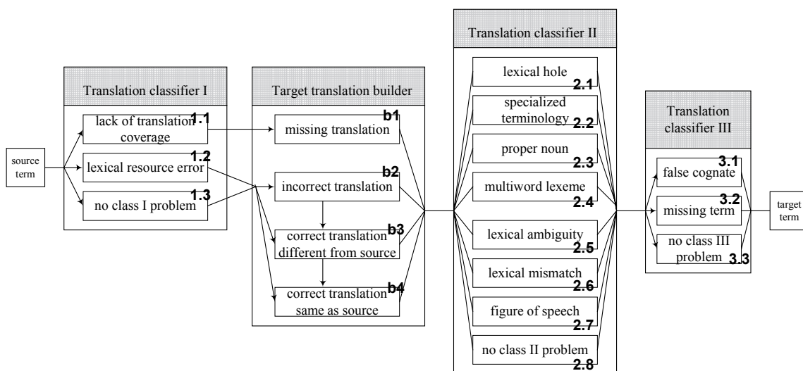
Figure 1: Translation taxonomy.
