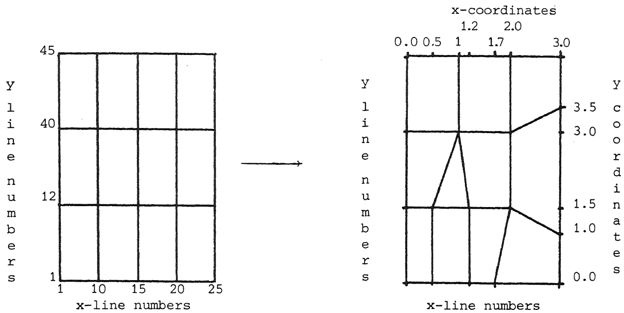
FIGURE 1. The mesh is specified in the SEMMY2 input language by: x(1) = 0, x(10) = 2 \cdot 0.5, 2 \cdot 1, x(15) = 2 \cdot 1.2, 2 \cdot 1, x(20) = 1.7, 3 \cdot 2, x(25) = 3, y(1) = 0, y(12) = 4 \cdot 1.5, 1, y(40) = 4 \cdot 3., 3.5, y(45) = 4.5.
